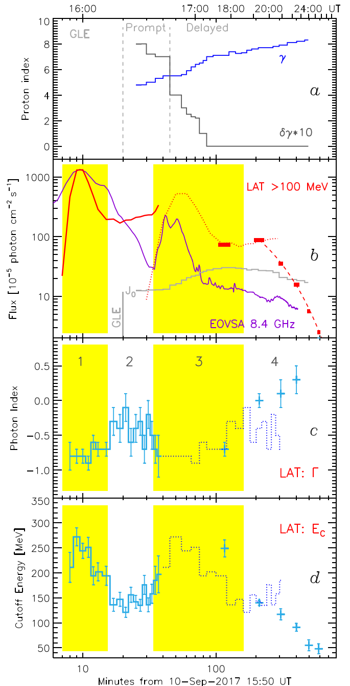
Figure 1. Two components of GLE (prompt and delayed) and four phases of the high-energy \gamma -ray emission (1–4) of the solar flare–CME eruption on 2017 September 10. (a) Time development of the GLE spectrum. The proton rigidity spectrum is of the form: J_{\parallel}(P) = J_0 P^{-\gamma + \delta\gamma(P-1 \text{ GV})} , where rigidity P is measured in GV, J_{\parallel} is the intensity of protons arriving from the Sun along the distribution symmetry axis. (b) The high-energy \gamma -ray profile observed with Fermi/LAT (red solid line and blocks, with data gaps caused by the orbit limitations), compared with the normalized profile of MW emission observed with EOVSA, and the GLE intensity magnitude J_0 (in units of 0.5 \text{ cm}^{-2} \text{ s}^{-1} \text{ sr}^{-1} \text{ GV}^{-1} ). (c), (d) The photon spectral index, \Gamma , and cutoff energy, E_c , of the best-fit \gamma -ray spectrum dN_{\text{ph}}(E)/dE = N_0 E^{\Gamma} \exp(-E/E_c) . Dotted profiles in (b)–(d) are for a possible interpolation through the data gap (explained in the text). The dashed red line in (b) is an exponential fit to the time profile of the \gamma -ray decay.
