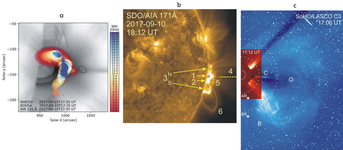
Figure 2. Flare–CME structures at around the peak time of the delayed \gamma -ray emission. (a) MW-emission frequency map by EOVSAs (color coded similarly to Yu et al. 2020) and the 6–12 keV X-ray map by RHESSI (black contours at 10%, 50%, and 90% of the maximum), superimposed on the SDO/AIA 131 Å image (gray) at the end of Phase 3 of the \gamma -ray flare. (b) The AIA 171 Å image at 18:12 UT. The main flare arcade (1) continuously rises up. The red circle specifies the 30–100 keV X-ray source location observed by RHESSI at 15:54 UT (the \gamma -ray Phase 1). The southern flare arcade (2) is seen in the soft X-ray images by GOES 15/Solar X-ray Imager already in Phase 1. In EUV images, its brightening expands to the south during Phase 2 and early Phase 3. In mid-Phase 3, the pair arcs (3) simultaneously brighten up to the north and the south of the main flare arcade. In Phase 4, the southern arcs (3S) exhibit numerous rapid evolutions (with no new brightening in soft X-rays). Also specified are the CME-trailing reconnection current sheet (4) with its southern extension (5; Chen et al. 2020b) and the high, rising loops (6) that disappear during Phase 4 at around 20:27 UT on 2017 September 10. (c) The Large Angle and Spectrometric Coronagraph Experiment (LASCO)/C3 image showing the CME core/magnetic flux rope (O), the bright blob (C) injected along the CME-trailing current sheet, and the southern CME loops (B). The blob leads a wider ejection seen in the 17:12 UT image by LASCO/C2 (red insert).
