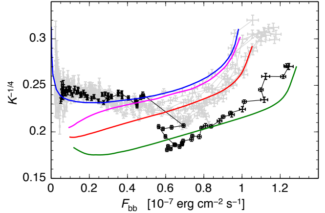
Figure 4. Black body normalization versus the flux of HETE J1900.1–2455 bursts observed with the PCA instrument, together with the theoretical color correction curves, f_c , for a M_{\text{NS}} = 1.4M_{\odot} and R_{\text{NS}} = 12 \text{ km} NS. The track from the 2005 July 21 burst is high-lighted with black color. The blue, purple, red and green lines are for MATMOS f_c curves with metal enhancement factors \zeta = 0.01, 1, 10 and 40 , respectively.
