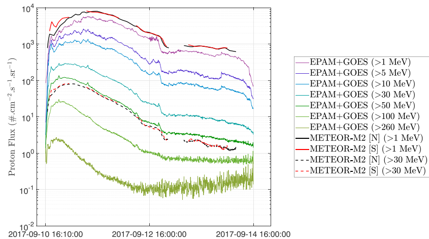
Figure 13. Integral fluxes derived from ACE/EPAM and GOES/EPEAD compared to data from two METEOR-M2 measurements in the northern and southern polar caps. ACE = Advanced Composition Explorer; EPEAD = Energetic Proton, Electron and Alpha Detector.
