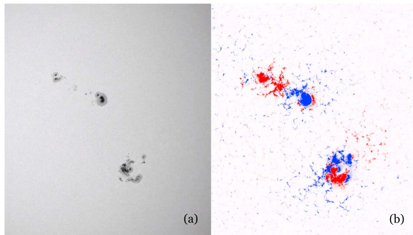
Figure 1. White light continuum image (a) and magnetogram image showing opposing polarities of the solar magnetic field in blue and red (b) recorded on 6 September 2017 as viewed by Solar Dynamics Observatory/Heliioseismic and Magnetic Imager showing AR 12674 (above) and AR 12673 (below). AR = Active Region.
