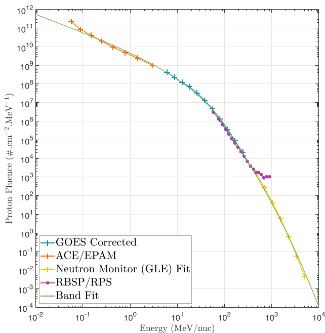
Figure 14. Full differential spectra for the solar particle event beginning on 10 September 2017 using data from ACE/EPAM and GOES-15/EPEAD and high-energy data determined from neutron monitor measurements. Data from the RBSP/RPS instrument are shown in purple and includes galactic cosmic ray fluxes. ACE = Advanced Composition Explorer; EPEAD = Energetic Proton, Electron and Alpha Detector; RBSP = Radiation Belt Storm Probes; GLE = ground level enhancement.
