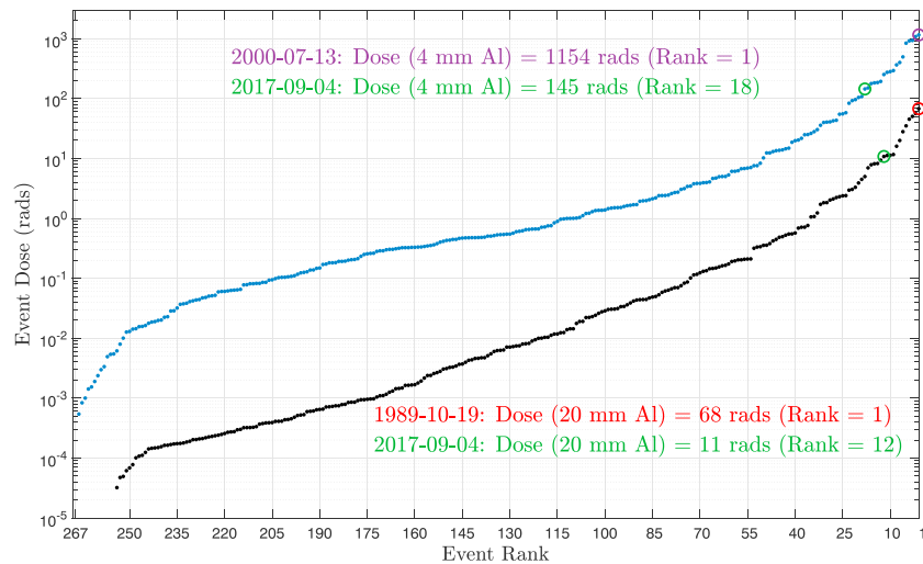
Figure 15. Cumulative distribution of ionizing dose levels calculated using SHIELDOSE behind aluminum shielding of 4 mm (blue dots) and 20 mm (black dots) for all solar particle events from 1974 until mid-2015 with the addition of the solar particle event of early September 2017.
