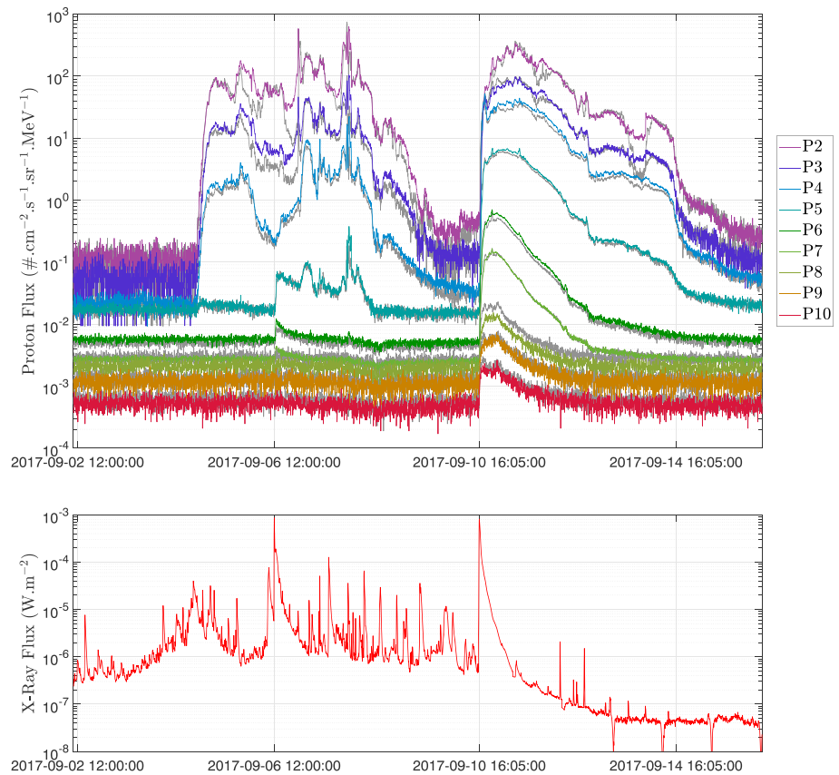
Figure 4. GOES-15/Energetic Particle Sensor differential fluxes from Energetic Proton, Electron and Alpha Detector west facing and High Energy Proton and Alpha Detector detectors (colored lines) and east facing detectors (gray lines) are shown in the top panel. GOES X-ray fluxes (1.0–8.0 Å) are shown in the bottom panel. Two vertical grid lines are selected to match the two X-class X-ray flare peaks to the nearest 5 min (the time resolution of the particle data); the two other vertical grid lines are 4 days before (after) these flare peaks.
