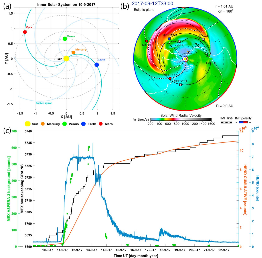
Figure 21. (a) The planet positions in the inner solar system on 10 September 2017, with the Parker spiral simulated for a solar wind speed of 400 km/s. (b) A still image from 12 September at 23:00 of the solar wind velocity in the ecliptic plane from a WSA-ENLIL + Cone model simulation (see Witasse et al., 2017, for references) showing the interplanetary coronal mass ejection shortly before it hit Mars on 13 September. The full simulations are available at http://ccmc.gsfc.nasa.gov (run number: Leila Mays 120817 SH 9; Lee et al., 2018). The colors represent the radial speed, as indicated in the color scale. (c) Some data acquired by satellites in orbit around Mars: in blue, the count rate of the HEND detector (scintillator block) on board Mars Odyssey (Boynton et al., 2004); in red, its cumulative number; in green, the background of the IMA (Ion Mass Analyser) sensor from the ASPERA-3 instrument on board Mars Express (Barabash & Lundin, 2006); and in black, a housekeeping parameter from Mars Express (EDAC error counter) sensitive to space weather events (Witasse et al., 2018). The space weather event is clearly identified with these data.
