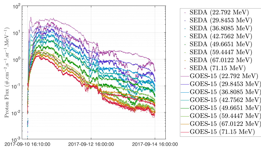
Figure 10. Data from Himawari-8/SEDA/PT (dots) compared to corrected GOES-15/EPEAD (lines) differential fluxes interpolated to SEDA channel mean energies. (n.b. The same colors are used for each energy for the different detectors). SEDA = Space Environment Data Acquisition; PT = Proton Telescope; EPEAD = Energetic Proton, Electron and Alpha Detector.
