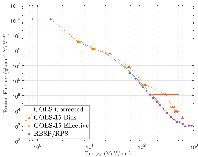
Figure 5. GOES-15/Energetic Particle Sensor differential fluxes with nominal energy bins are shown in red, the Energetic Proton, Electron and Alpha Detector bin effective energies as presented by Sandberg et al. (2014) are shown with yellow triangles, and the resulting spectrum is shown with the blue line. Data from the RBSP/RPS instrument are shown in purple.
