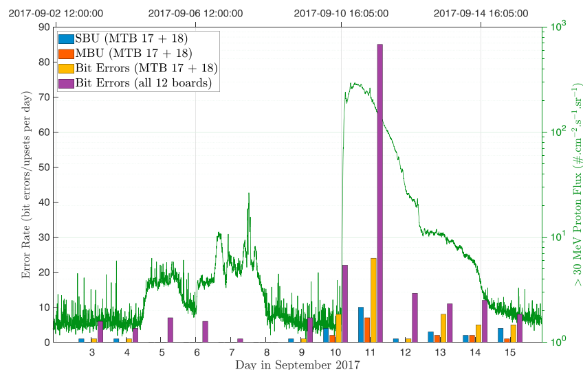
Figure 16. Single (SBU) and Multiple (MBU) Bit Upsets and total bit errors in two memories on the Memory Test Board (MTB) flying on Alphasat plus the total bit errors on a total of 12 memories for each day from 3 to 15 September 2017. Also plotted is the > 30-MeV proton flux that has been calculated from GOES/EPEAD data as given in Figure 13. EPEAD = Energetic Proton, Electron and Alpha Detector.
