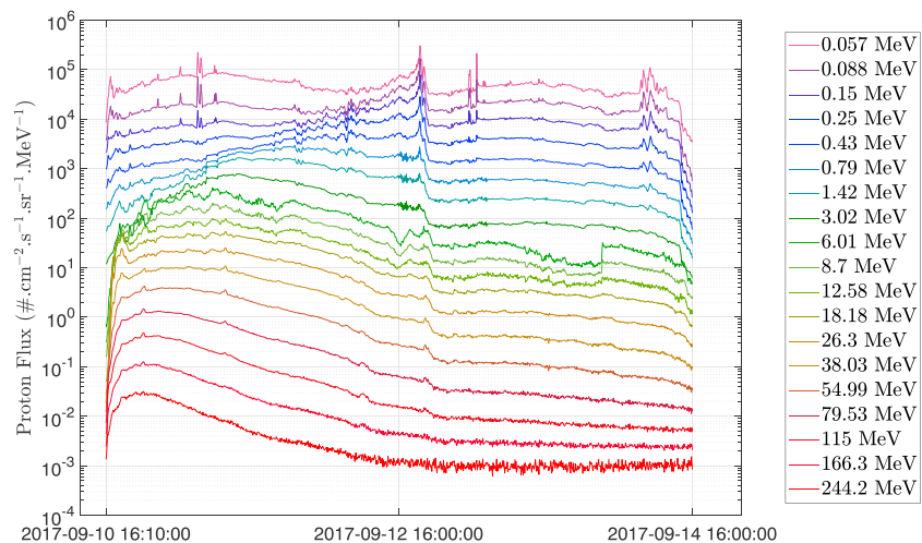
Figure 12. Differential fluxes from ACE/EPAM and GOES/EPEAD. The first eight energies (up to 3.02 MeV) are taken from the EPAM instrument fluxes, while the last 11 channels (6.01 MeV and above) are taken from the (corrected) EPEAD instrument fluxes. ACE = Advanced Composition Explorer; EPEAD = Energetic Proton, Electron and Alpha Detector.
