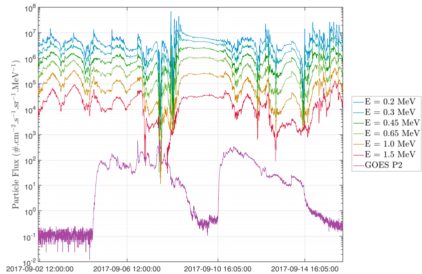
Figure 11. Data from Himawari-8/SEDA/SURF electron detector compared to corrected GOES-15/EPEAD differential fluxes in P2 (4–9 MeV). SEDA = Space Environment Data Acquisition; EPEAD = Energetic Proton, Electron and Alpha Detector.
