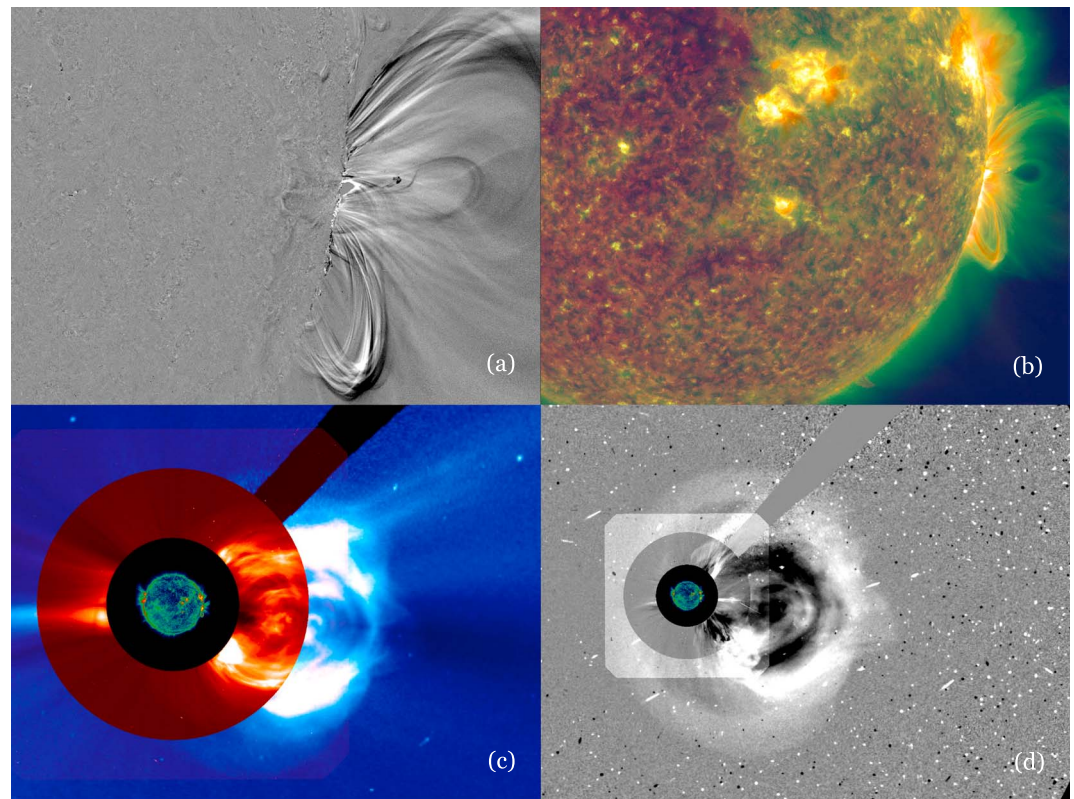
Figure 3. Images of the X8.2 flare and associated CME from 10 September 2017 with increasing field of view: difference image of the flare and CME as viewed by SDO/AIA in 171-Å wavelength (a); composite image of the southwest region of the solar disc at the time of the flare as viewed by SDO/AIA in 171-, 211-, and 304-Å wavelengths (b); high-contrast SDO/AIA 171 Å and SOHO/LASCO C2 and C3 coronagraph images extending to 11 solar radii centered around 16:15 UTC (c); high-contrast SDO/AIA 171 Å and SOHO/LASCO C2 and C3 difference images from 16:30 to 16:40 UTC extending to 22 solar radii (d) showing particle hits on the coronagraph images (solar north on all images is vertical upward direction). CME = coronal mass ejection; SDO = Solar Dynamics Observatory; AIA = Atmospheric Imaging Assembly; SOHO = Solar and Heliospheric Observatory; LASCO = Large Angle and Spectrometric Coronagraph.
