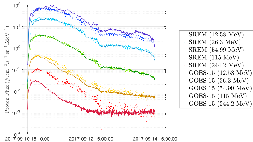
Figure 7. Corrected GOES-15/EPEAD differential fluxes compared to Level 2 data from Proba-1/SREM at five interpolated energies. EPEAD = Energetic Proton, Electron and Alpha Detector; SREM = Standard Radiation Environment Monitor.
