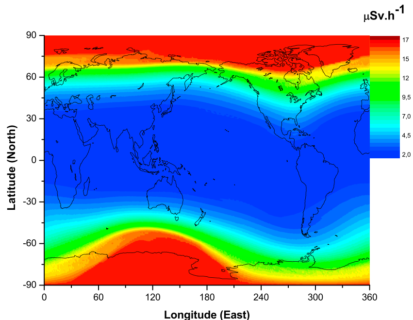
Figure 20. Doses at an aircraft altitude of 40,000 feet (12.2 km) above sea level during the peak high-energy intensity of the September 2017 SPE (GLE 72). SPE = solar particle event; GLE = ground level enhancement.
