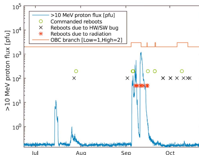
Figure 18. The GOES-15/EPEAD > 10-MeV proton flux, the Aalto-1 OBC branch in use, and the reboots of the Aalto-1/OBC. OBC = onboard computer. EPEAD = Energetic Proton, Electron and Alpha Detector.
