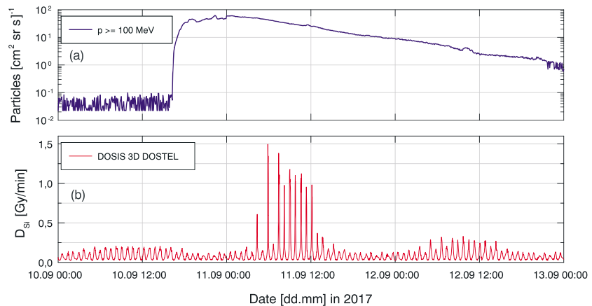
Figure 19. (a) GOES-15 proton flux > 100 MeV; (b) DOSIS 3D DOSTEL absorbed dose rate (in Si) for 10–13 September 2017. Note that relevant contributions from the South Atlantic anomaly crossings have been removed based on the procedure given in Berger et al. (2018)
