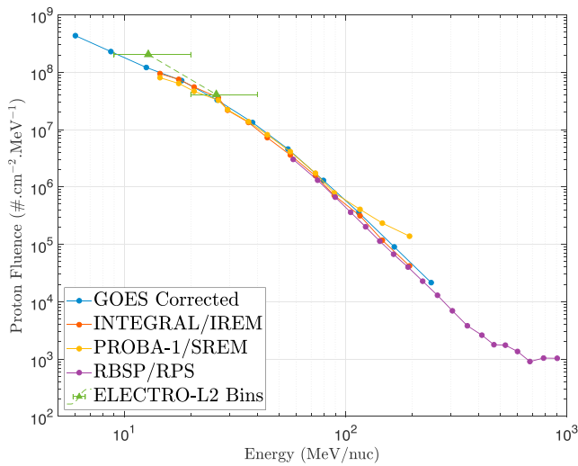
Figure 9. Differential fluence spectra of GOES-15/EPEAD compared to INTEGRAL/IREM, PROBA-1/SREM and ELECTRO data. Data from the RBSP/RPS instrument is shown in purple. EPEAD = Energetic Proton, Electron and Alpha Detector; INTEGRAL = INTERNATIONAL Gamma-Ray Astrophysics Laboratory; SREM = Standard Radiation Environment Monitor; RBSP = Radiation Belt Storm Probe.
