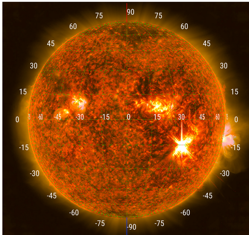
Figure 2. Composite image of onset of X9.3 flare recorded on 6 September 2017 as viewed by Solar Dynamics Observatory/Atmospheric Imaging Assembly in 171- and 304-Å wavelengths. The flare peak (as measured by the maximum X-ray flux in the 1- to 8-Å range) occurred at 12:02 UTC (solar north and south are indicated by the red and blue vertical line segments, respectively).
