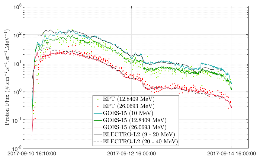
Figure 8. Corrected GOES-15/EPEAD differential fluxes compared to data from Proba-V/EPT and ELECTRO-L2 data interpolated to estimated ELECTRO-L2 mean energies. EPEAD = Energetic Proton, Electron and Alpha Detector; EPT = Energetic Particle Telescope.
