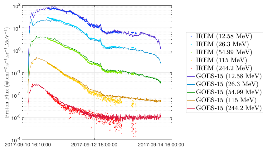
Figure 6. Corrected GOES-15/EPEAD differential fluxes compared to Level 2 data from INTEGRAL/IREM at five interpolated energies. EPEAD = Energetic Proton, Electron and Alpha Detector; INTEGRAL = INTErnational Gamma-Ray Astrophysics Laboratory; IREM = INTEGRAL Radiation Environment Monitor.
