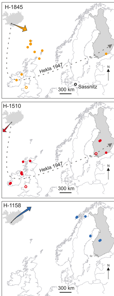
Figure 8. Maps showing the occurrence of Hekla 1845, Hekla 1510 and Hekla 1158 tephra in Northern Europe. Circles mark tentative correlations and dots geochemically confirmed cryptotephra deposits or contemporary eyewitness reports of fall-out. Axes of tephra fall within Iceland are from Larsen et al. , 1999 and Guðnason et al. , 2018. The arrow marking the main dispersal axis of Hekla 1947 tephra based on prevailing wind directions is from Salmi (1948). Data for sites of cryptotephra detection and eyewitness reports are from Dugmore et al. , 1995; Pilcher et al. , 1996; Wastegård, 2002; Pilcher et al. , 2005; Balascio et al. , 2011; Reilly and Mitchell, 2015; Watson et al. , 2015, 2016 and 2017; Guðnason et al. , 2018; Cooper et al. , 2019b. [Color figure can be viewed at wileyonlinelibrary.com ]
