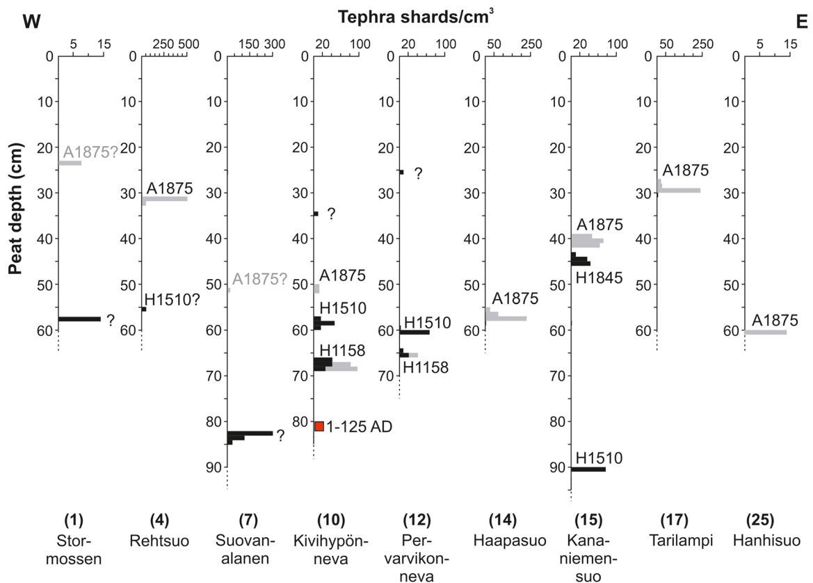
Figure 5. Tephra shard concentration profiles for the peatland sites in this study. Deposits consisting of colourless shards are marked in grey and brownish shards in black. The red square marks the position of the radiocarbon-dated peat sample. Unidentified layers are labelled with a question mark. [Color figure can be viewed at wileyonlinelibrary.com ]
