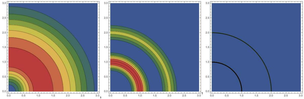
Figure 2: Sum |\langle \alpha | n' \rangle|^2 + |\langle \alpha | n'' \rangle|^2 with n' = 1 and n'' = 4 for N = 1, 10, 1000 (left to right): Contourplot on part of \mathcal{M} , which is now the complex plane (values increase from blue to red).
