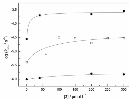
Fig. 3 Logarithmic pseudo first-order rate constants for the cleavage of 4a ( \square ), 4b ( \bullet ) and 4c ( \blacksquare ) as a function of the concentration of the Zn^{II} complex of the cleaving agent 2 at 90 °C, pH = 7.42, I(\text{NaClO}_4) = 0.10 \text{ mol L}^{-1} , [4a] = [4b] = [4c] = 5.0 \mu\text{mol L}^{-1} .
