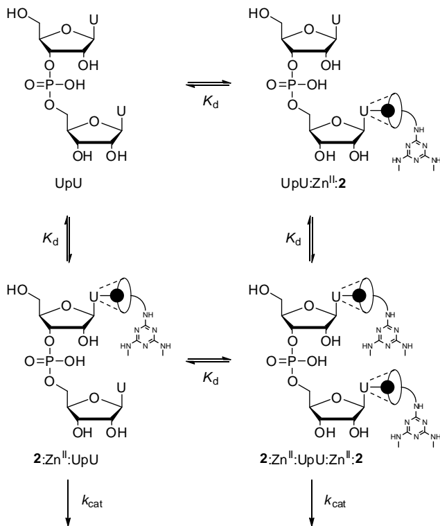
Scheme 5 Complexation equilibria and reactive complexes of UpU and Zn^{II}:2 .
