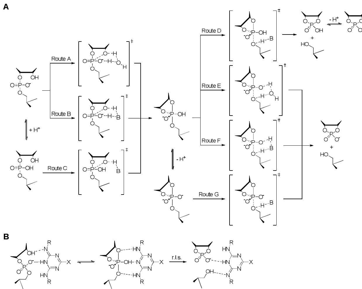
Scheme 1 Proposed mechanisms for RNA cleavage catalyzed by general acids and bases.
