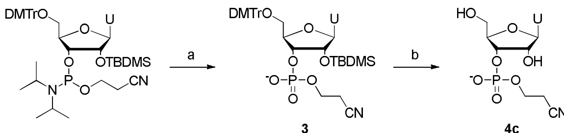
Scheme 3 Preparation of the alkyl esters of uridine-3'-phosphate. Reagents and conditions: (a) 1. H 2 O, 4,5-dicyanoimidazole, MeCN, 2. I 2 , H 2 O, pyridine, (b) 1. Et 3 N·3HF, THF, 2. HCl, MeOH, CH 2 Cl 2 .
