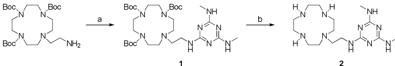
Scheme 2 Preparation of the cleaving agent. Reagents and conditions: (a) 1. cyanuric chloride, DIPEA, MeCN, 2. methylamine, EtOH, MeCN, (b) 1. TFA, CH 2 Cl 2 , MeOH, 2. Dowex 1x2 (OH).
