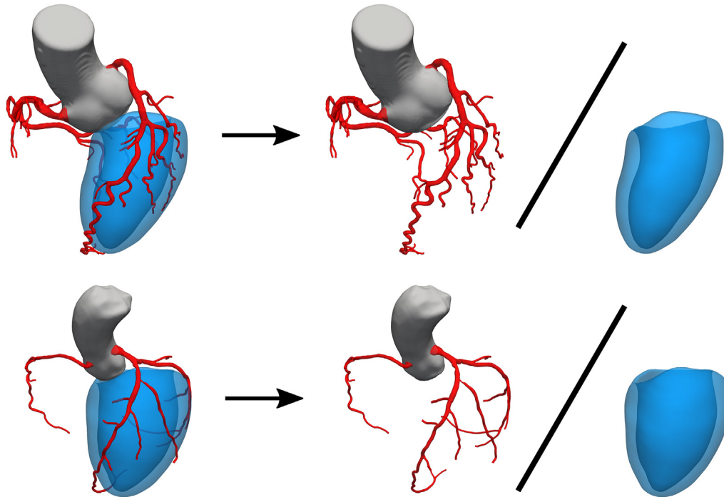
Figure 1. Graphical presentation of the coronary artery volume and left ventricular myocardial mass and the coronary volume to left ventricular mass ratio showing the difference between a non-diabetic (top of figure) and a diabetic patient (bottom of figure). Both subjects had non-obstructive coronary artery disease (0–30% diameter stenosis).
