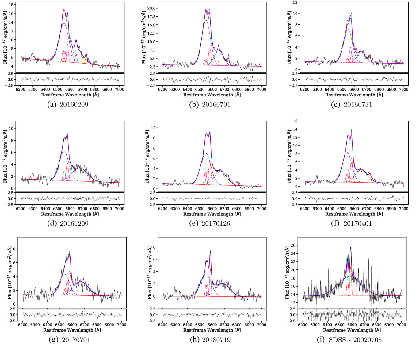
Figure A2. Evolution in time of the H\alpha line region with the fit to the various components with multiple Gaussian curves. In all the panels, the red dashed lines are the two [N\ II] lines, the blue dashed lines are the two H\alpha components, the magenta dashed line is the H\alpha narrow component, the brown dashed line is the He\ I line (only present in the first two panels a and b), and the orange dashed line is the blend of the two [S\ II] lines. Panel h is the spectrum taken after the object returned to its pre-outburst state, according to the Gaia light curve.
