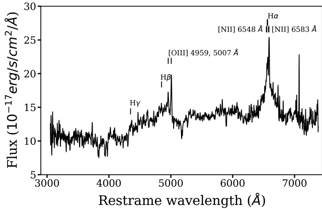
Figure 2. Archival spectrum from the SDSS legacy survey. The object shows broad Balmer emission lines and narrow forbidden oxygen and nitrogen lines.
