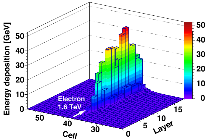
Fig. 26. Example of a 1.6TeV electron shower in the ECAL. Most of the shower energy is deposited along the shower axis near the shower maximum. For high energy showers ( > 500\text{GeV} ), some of the amplitudes are saturated, for example, those shaded in red.
