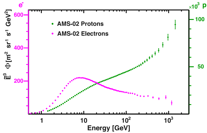
Fig. 64. The measured proton spectrum ( \bar{E}^3 \Phi_p , green, right axis) compared to the electron spectrum ( \bar{E}^3 \Phi_{e^-} , purple, left axis) - converted from measured rigidity to total energy for protons. The electron spectrum shows a distinctly different behavior from the proton spectrum over the entire energy range.
