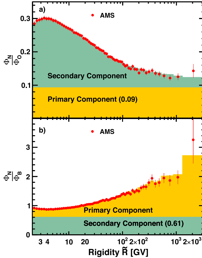
Fig. 95. (a) The AMS \Phi_N / \Phi_O ratio as a function of rigidity. (b) The AMS \Phi_N / \Phi_B ratio as a function of rigidity. The contributions of the primary and secondary components are indicated by the yellow and green shading, respectively. As seen from (a) and (b), the contribution of the secondary component in the nitrogen flux decreases, and the contribution of the primary component correspondingly increases, with rigidity.
