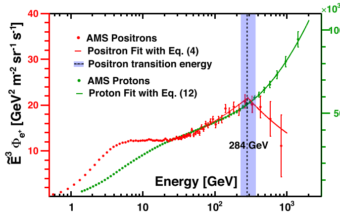
Fig. 66. The positron ( \tilde{E}^3\Phi_{e^+} , red data points, left axis) and proton ( \tilde{E}^3\Phi_p , green data points, right axis) spectra. Also shown are the fits of Eq. (4) to positron data and Eq. (12) to proton data. The dashed vertical line and the blue band show the positron transition energy and its uncertainty (see Section 2).
