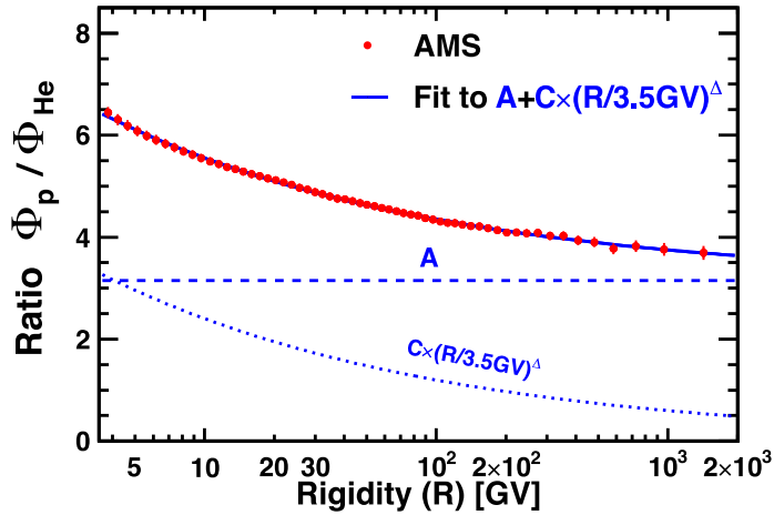
Fig. 80. The rigidity dependence of the proton-to-helium flux ratio together with a fit of the function A + C(R/3.5 \text{ GV})^\Delta (solid curve). The soft component, C(R/3.5 \text{ GV})^\Delta (dotted curve), and the helium-like component, A term (dashed line), are also shown.
