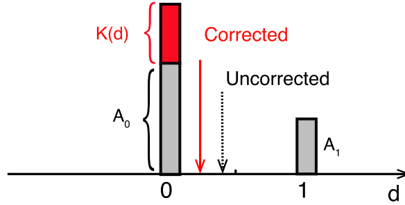
Fig. 5. Schematic of particle coordinate measurement in the silicon tracker. The solid red arrow indicates the point where the particle intersected the silicon sensor, the two adjacent strips are positioned at 0 and 1 in “strip” units. The maximum amplitude is defined as A_0 (at 0) and the next largest adjacent strip as A_1 (at 1). For an ideal tracker, the ratio between amplitude A_0 and A_1 gives the particle coordinate, d = 1/(1 + A_0/A_1) . To correct for the non-linear effect, the correction function K(d) is added to the measured non-linear amplitude A_0 . The dashed arrow shows the uncorrected coordinate measurement. The corrected coordinate is at its true position within the measured accuracy of few microns.
