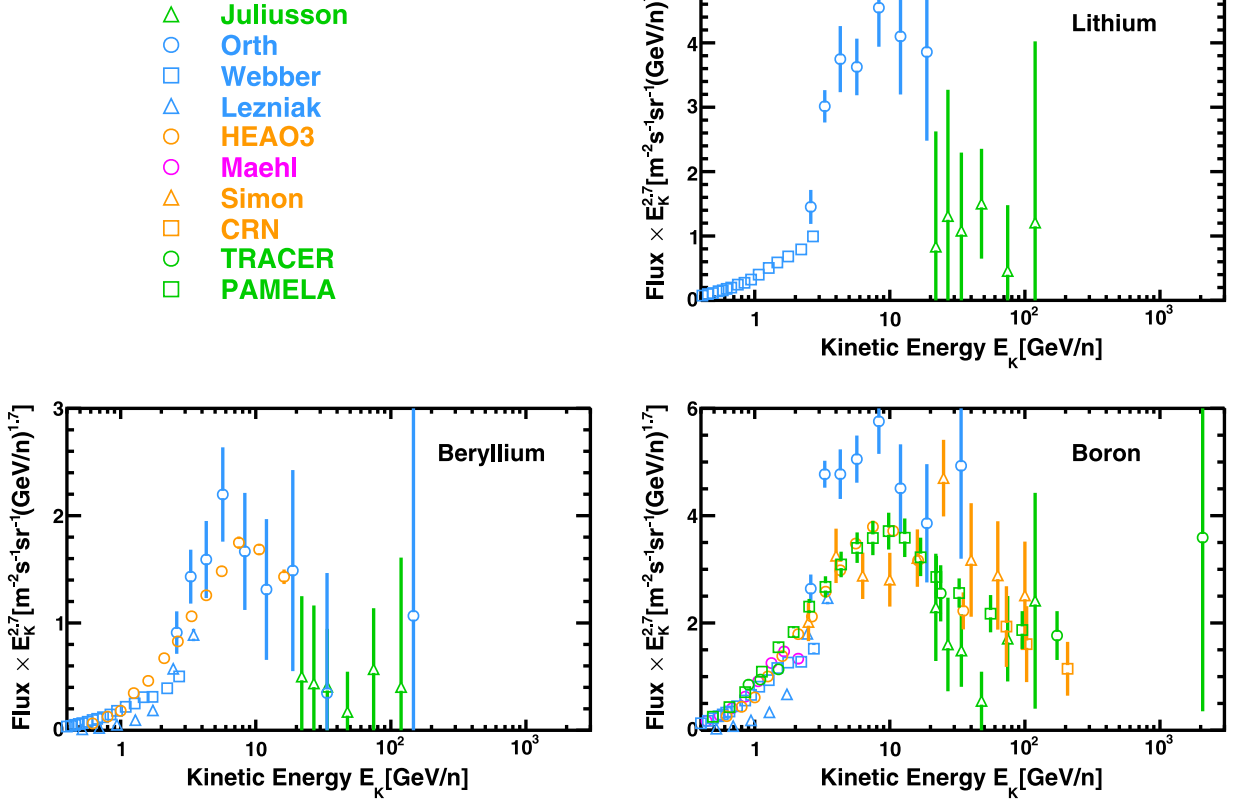
Fig. 81. The measurements of the lithium, beryllium, and boron fluxes [127–136] available before AMS as functions of kinetic energy per nucleon E_k multiplied by E_k^{2.7} .
