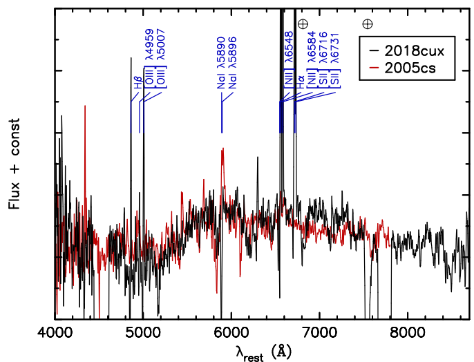
Fig. 7. SALT spectrum (black) at the location of AT 2018cux corrected for host galaxy extinction of A_V = 2.1 mag. The overlaid (red) +106 d spectrum of the subluminal Type IIP SN 2005cs (Pastorello et al. 2009) is shifted with an arbitrary added constant and shows overall similarity to that of the AT 2018cux observations. The spectra have been redshift corrected to rest frame. The most prominent host lines of NGC 3256 are indicated. The main telluric bands are marked with a \oplus symbol.
