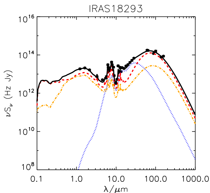
Fig. 15. An example SED fit (solid black curve) to the data of one of the sample LIRGs, IRAS 18293-3413 (points), with a combination of a starburst (dashed red), a spheroidal galaxy (dot-dashed orange), and an AGN (dotted blue) component.
