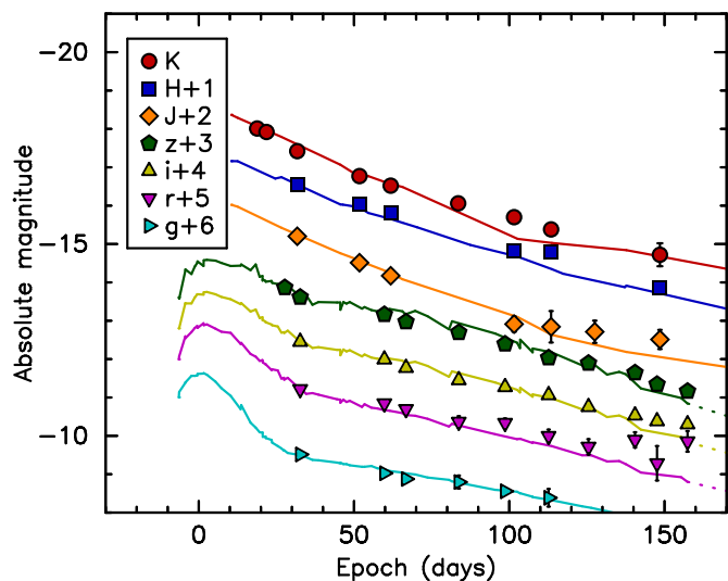
Fig. 2. Absolute magnitude light curves of SN 2018ec after correcting for host extinction ( A_V = 2.1 mag). The light curves of the Type Ic SN 2007gr are shown with solid lines and shifted vertically by -0.58 mag (optical light curves extrapolated with linear fits for comparison are indicated with dotted curves). The estimated errors for most light curve points are smaller than the symbol size. The epoch 0 is the B -band maximum estimated for SN 2007gr by Hunter et al. (2009).
