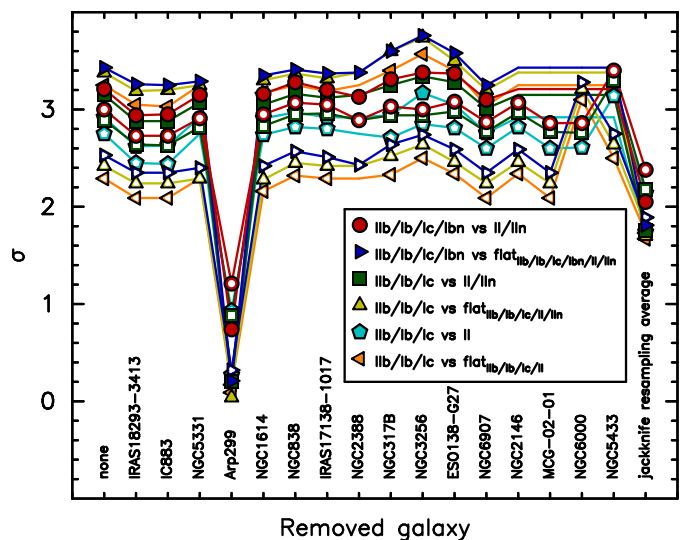
Fig. 17. Yielded \sigma values from a selection of statistical tests for the sample with individual galaxies and their sample CCSNe removed from the analysis as a test. While removing individual galaxies and thus typically only 1 or 2 CCSNe from the sample will not have a major effect on the resulting AD test values, the arbitrary removal of Arp 299 and its 6 Type IIb/Ib SNe would make the discussed trends nonexistent. Open and closed symbols show the values for samples with the host SNR of \geq 0.0 and \geq 0.5 \text{ CCSN yr}^{-1} , respectively. Data points are not shown in cases where the removal of the galaxy is irrelevant for the comparison between the analysed samples. With the large number of hosted sample CCSNe, the removal of the LIRG Arp 299 with a yielded young starburst age has also the largest weight in the jackknife resampling averages of the p -values for each set of comparisons, and result in mean values of \theta_p \geq 0.017 ( \leq 2.4 \sigma ).
