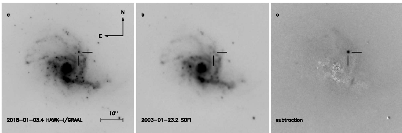
Fig. 1. a) 1' \times 1' subsection of the HAWK-I/GRAAL K_s -band discovery image of SN 2018ec in NGC 3256, b) SOFI reference image, and c) a subtraction between the images. The AO enhanced HAWK-I/GRAAL image with FWHM \sim 0''.4 has a superior image quality compared to the normal ground-based seeing SOFI image with FWHM \sim 0''.8 . The location of SN 2018ec is shown with tick marks in all the panels; the orientation and image scale are indicated in the first panel.
