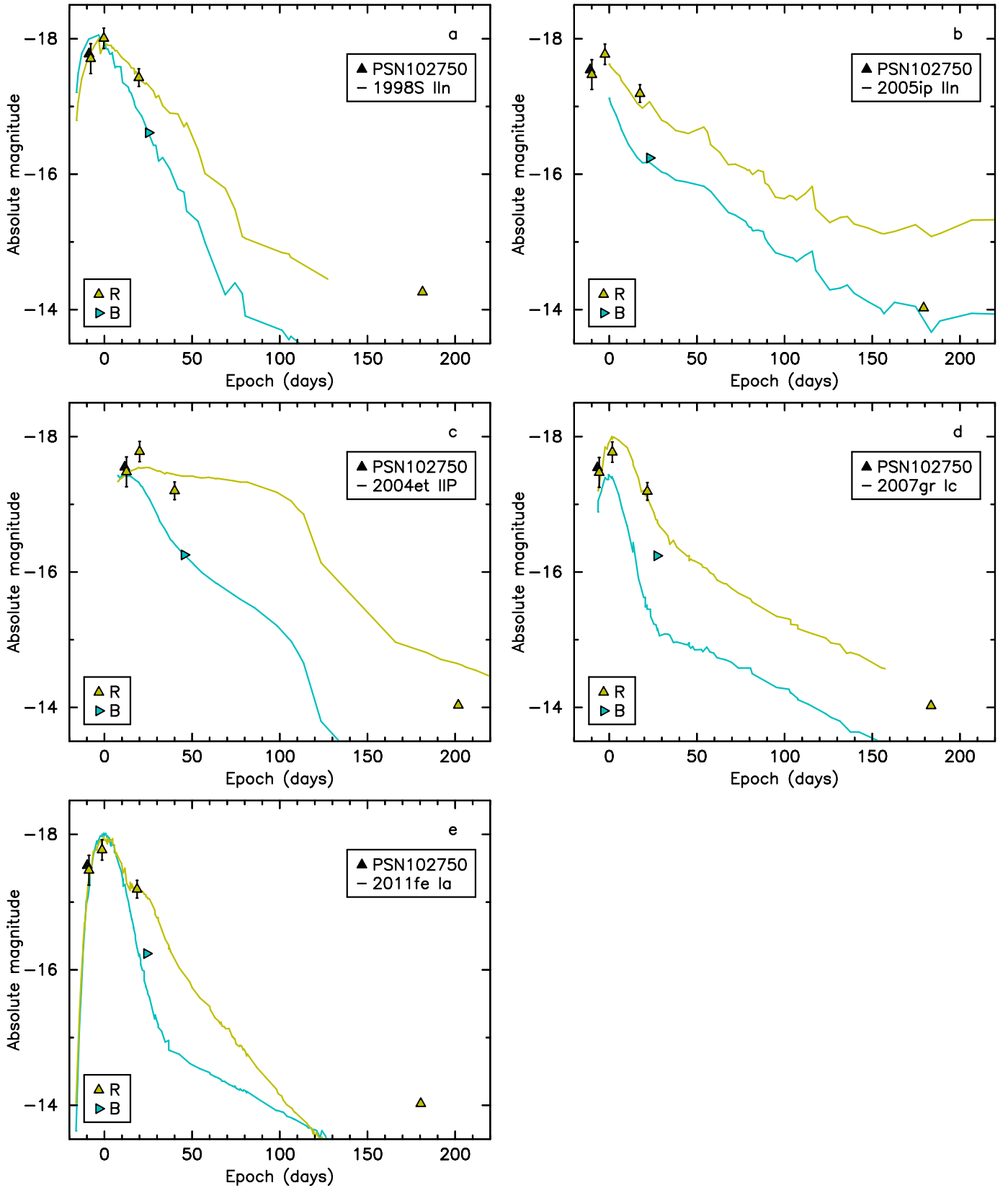
Fig. 9. PSN102750 light curve comparisons to those of a) Type II SN 1998S, b) Type II SN 2005ip, c) Type IIP SN 2004et, d) Type Ic SN 2007gr, and e) Type Ia SN 2011fe. The reported unfiltered discovery magnitude is also shown in the plot with a black symbol.
