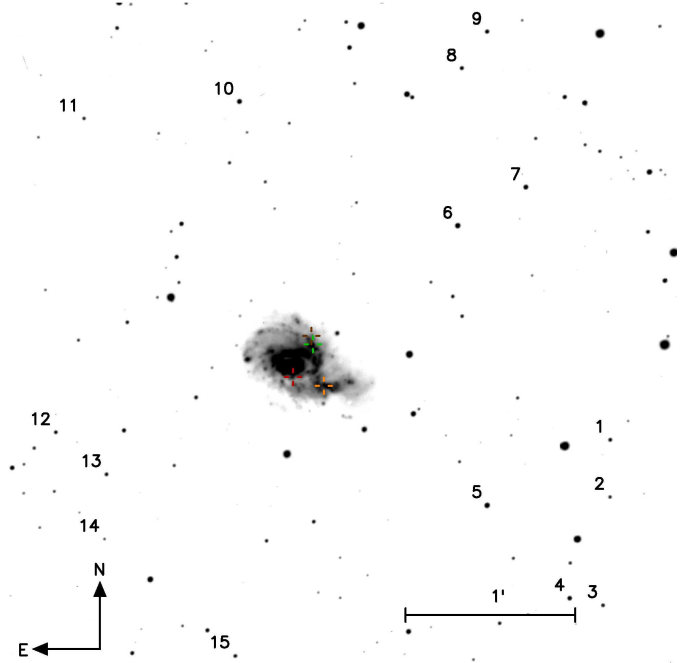
Fig. A.1. 4' \times 4' ePESSTO NTT+EFOSC2 r -band image of the field of NGC 3256 on 2018 January 16. The locations of sequence stars, SN 2018ec (green), AT 2018cux (red), PSN102750 (brown), and SN 2001db (orange) are indicated. North is up, east is left.
