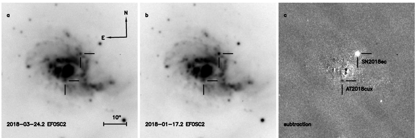
Fig. 5. a) 1' \times 1' subsection of the EFOSC2 i -band discovery image (FWHM \sim 0''.9 ) of AT 2018cux in NGC 3256, b) pre-discovery EFOSC2 reference image (FWHM \sim 0''.8 ), and c) a subtraction between the images. The locations of SN 2018ec and AT 2018cux are shown with tick marks in all the panels. Since the reference image contains increased flux from SN 2018ec compared to that of the AT 2018cux discovery image, the colour scale of the two events is reverse in the subtraction. The image scale and orientation are indicated in the left panel.
