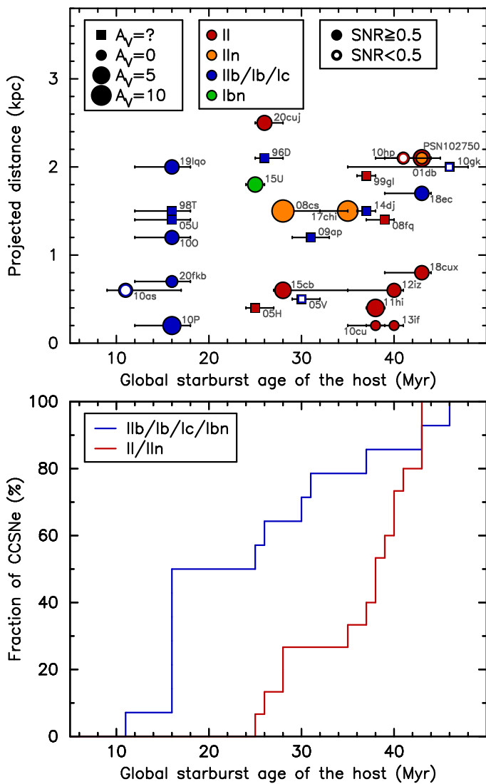
Fig. 16. Upper panel: Type distribution of classified CCSNe compared to our SED modelled global age of the host starburst at the central regions of our sample LIRGs. The sizes of the symbols indicate the derived host galaxy extinction of the SNe, with unknown (and likely small) extinction cases indicated with square symbols. The symbol colours indicate the CCSN subtype classifications. The events are marked with closed and open symbols based on their estimated host CCSN rate above and below 0.5 \text{ CCSN yr}^{-1} , respectively. Lower panel: A simplified cumulative distribution presentation of the upper panel data of the Type IIb/Ib/Ic/Ibn and Type II/IIIn samples of CCSNe. The data suggests that H-poor and H-rich CCSNe come from very young ( \lesssim 30 \text{ Myr} ) and older ( \gtrsim 30 \text{ Myr} ) starbursts, respectively.
