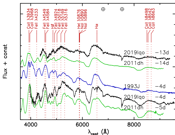
Fig. 12. The spectra of SN 2019lqo compared to those of Type IIb SNe 2011dh (Ergon et al. 2014) and 1993J (Matheson et al. 2000). The most prominent SN lines are indicated based on Ergon et al. (2014). The spectra have been extinction and redshift corrected, and shifted vertically for clarity. The main telluric band wavelengths for SN 2019lqo are indicated with a \oplus symbol.
