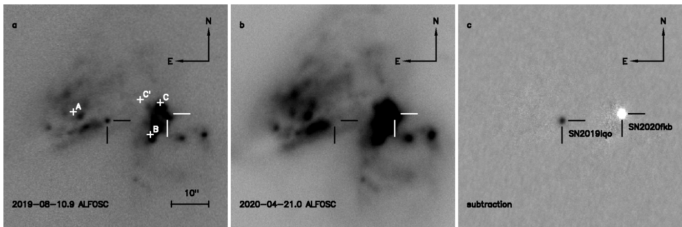
Fig. 10. a) 1' \times 1' subsection of a NOT V-band follow-up image of SN 2019lqo in Arp 299, b) follow-up image of SN 2020fkb, and c) a subtraction between the images. Tick marks indicate the locations of SNe 2019lqo and 2020fkb. The image scale and orientation are indicated in the left panel. The marked locations of IR bright main components (A, B, C, C') of Arp 299 (Gehrz et al. 1983) illustrate that some of these regions are obscured in optical wavelengths.
