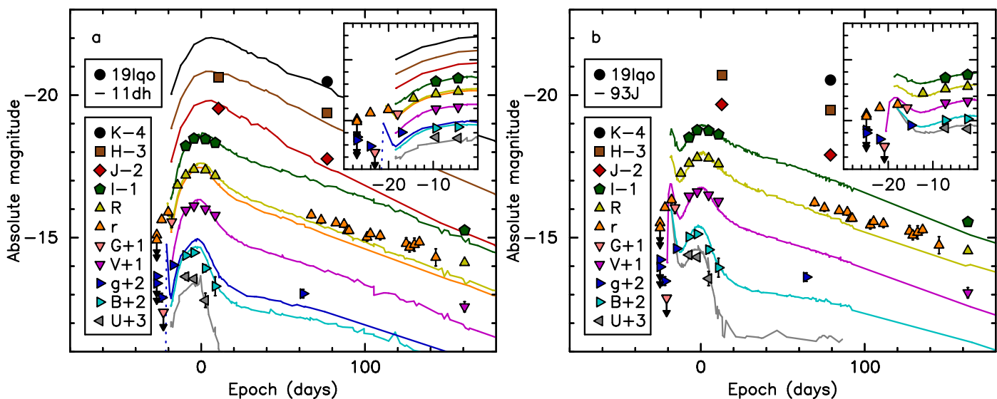
Fig. 11. SN 2019lqo light curve fits to Type IIb SNe a) 2011dh and b) 1993J. The inset zoom-in panels show the pre-maximum light curves suggesting a relatively long shock cooling phase. As previously noted, the Gaia G -band upper limit is probably optimistic. The epoch 0 is set to the estimated R -band peak.
