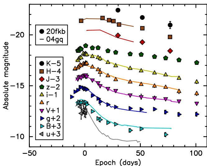
Fig. 13. SN 2020fkb absolute magnitude light curve (points) with an estimated host galaxy extinction of A_V = 0.4 mag yielded with a fit to Type Ib SN 2004gq, shown with solid lines and shifted vertically by +0.13 mag. The epoch 0 is set to the estimated V-band maximum.
