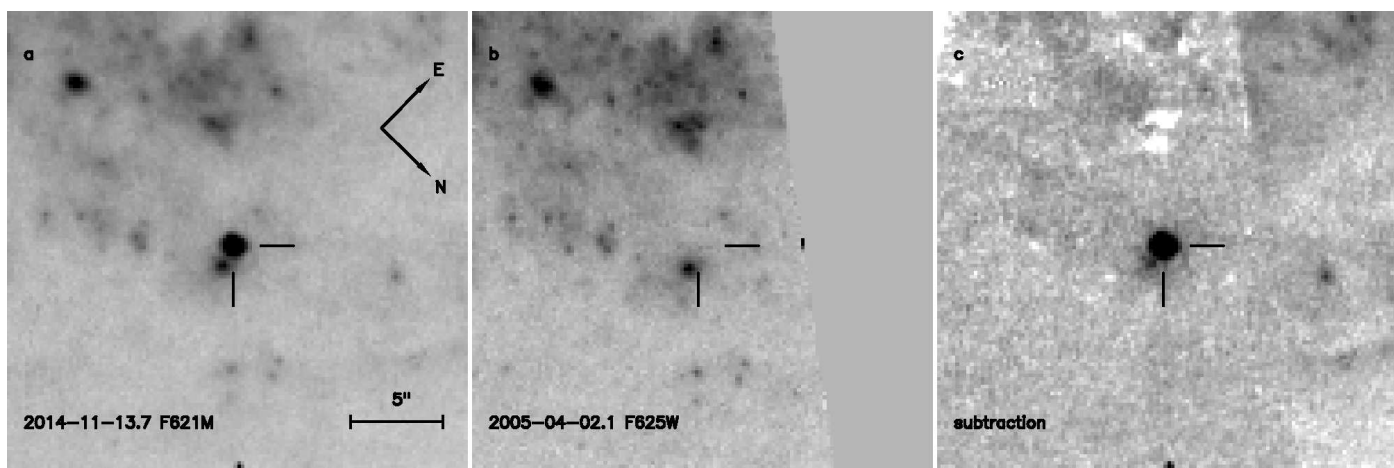
Fig. 8. a) Late-time HST F621M image of PSN102750 observed 190 d after the discovery of the transient, b) pre-explosion HST F625W image of the field of the transient, and c) a subtraction between the images. In addition to the event, the subtraction results also in some faint residuals from sources in the field likely due to the somewhat different filter widths of the two epochs of observations. The transient location is shown with tick marks. The orientation and image scale are indicated in the left panel.
