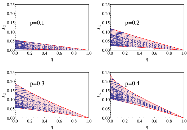
FIG. 6: (Color online) Illustration of the dependance of the minimal eigenvalue \lambda_G of operator G on the parameter q depicted for different values of the remaining parameters s, \alpha, \beta, \gamma, \theta and p .
