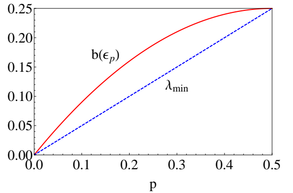
FIG. 4: (Color online) The strict difference between the boundariness b (upper line) and minimal eigenvalue \lambda_{\min} (lower line) for erasure channels is illustrated. Let us stress that the difference is not negligible and it is maximal for value p = 1/4 .
