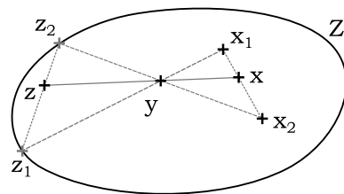
FIG. 2: Illustration of the proof of the Lemma 1
