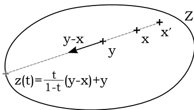
FIG. 1: Illustration of elements z and x' emerging in the definition of the weight function t_y(x) and in the property t_y(x') \leq t_y(x) , respectively.
