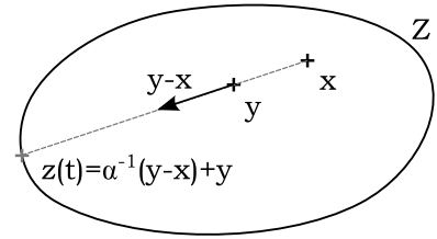
FIG. 5: The scalar \alpha extending y - x from the starting point y to the boundary coincides with the Minkowski gauge P_{Z-y}(y - x) and the decomposition of y with respect to this boundary point and x gives the value t_y(x) of the weight function.
