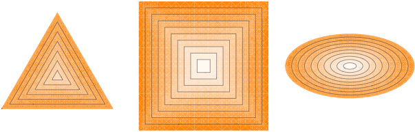
FIG. 3: (Color online) Contour plots of boundariness for simple convex sets. Let us note that the maximal value of boundariness is not the same in all of them.
