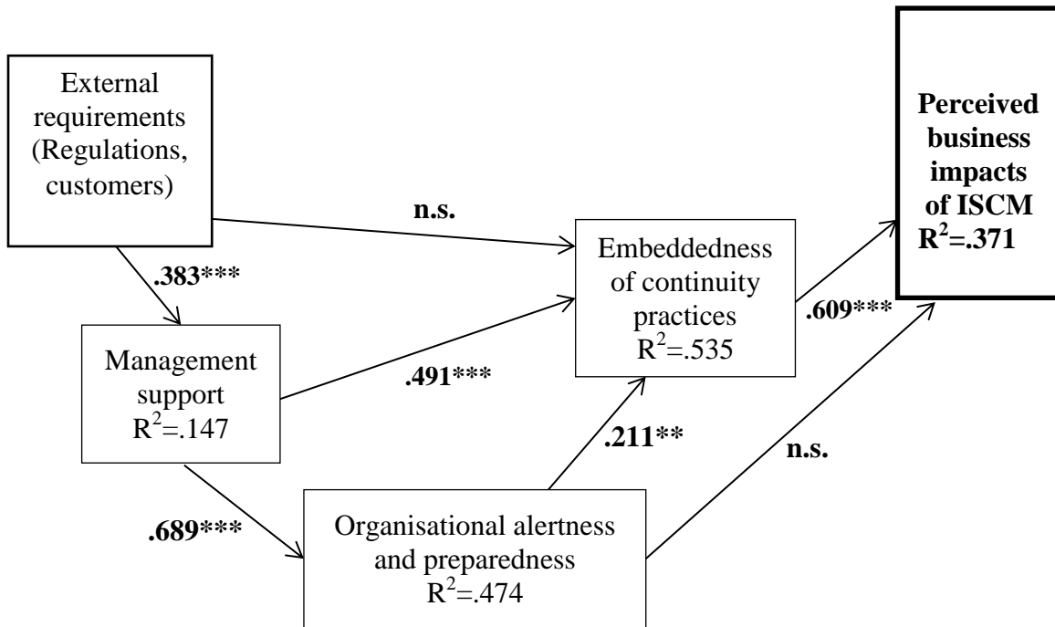
Figure 2. The test results: ** t > 1.96 , *** t > 2.576
