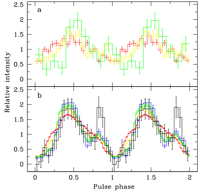
Fig. 2. Pulse profiles of IGR J19294+1816 obtained with NuSTAR in different energy bands during low (panel a) and high (panel b) states. Different colors correspond to different energy bands: 3–10 keV (red), 10–18 keV (yellow), 18–27 keV (green), 27–37 keV (blue), 37–50 keV (black).
