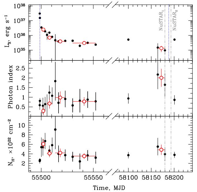
Fig. 1. Top panel: bolometrically corrected light curve of IGR J19294+1816 obtained with the Swift /XRT telescope in 2010 (left side) and 2017–2018 (right side) assuming distance to the source 11 kpc. Blue dotted lines show moments of periastron passages (see Sect. 3.4). Middle and bottom panels: corresponding evolution of the power law photon index and absorption value assuming an absorbed power law model. Black points correspond to individual XRT observations, whereas red open circles represent parameters obtained from the averaging of a few nearby observations with low count statistics. Vertical dash-dotted lines show moments of the NuSTAR observations.
