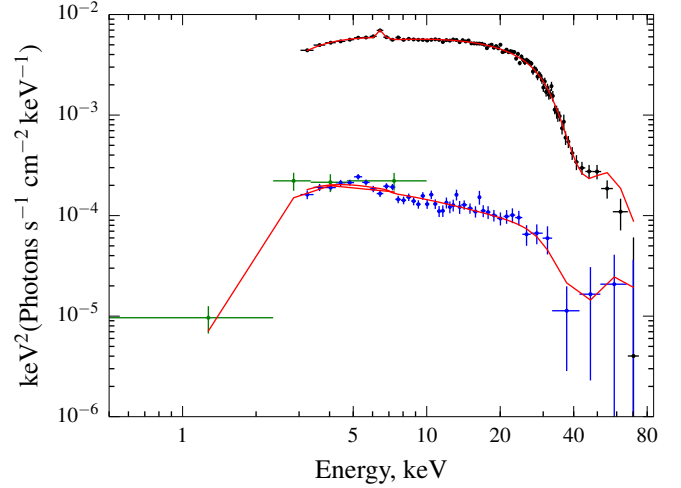
Fig. 5. Spectral energy distribution of IGR J19294+1816 obtained with the Swift /XRT and NuSTAR telescopes during the high (black dots) and low (blue and green dots) intensity states. The data from the two NuSTAR units are added together for plotting (but not for actual fit). Solid lines represent best-fit models for each observation including fundamental line only (see text).
