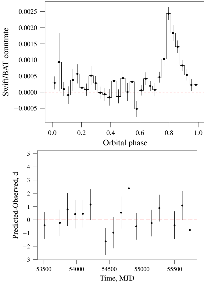
Fig. 8. Top panel: folded light curve of the source as observed by Swift /BAT. The zero phase here is arbitrary to make the peak clearly visible. Bottom panel: residuals to the linear fit of the outburst peak times determined as described in the text.
