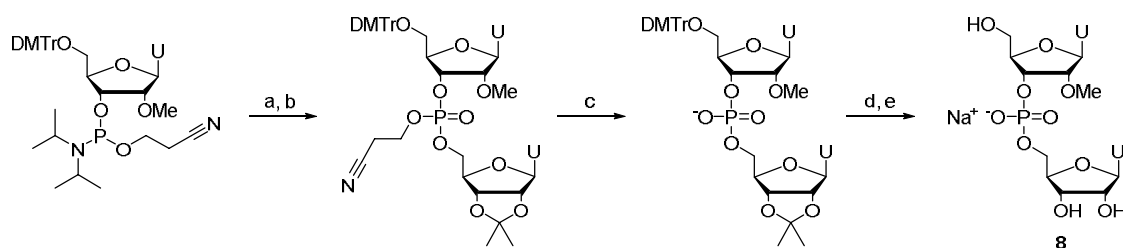
Scheme 4 Preparation of 2'- O -methyluridylyl-3',5'-uridine ( 8 , mUpU ). Reagents and conditions: (a) 2',3'- O -isopropylideneuridine, 1 H -tetrazole, MeCN, (b) I 2 , 2,6-lutidine, THF, H 2 O, (c) NH 3 , MeOH, (d) HCl, H 2 O, (e) Dowex 50Wx8 (Na + ), H 2 O.
