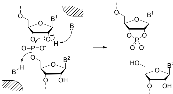
Scheme 2 General acid/base-catalyzed cleavage of RNA phosphodiester bonds.
