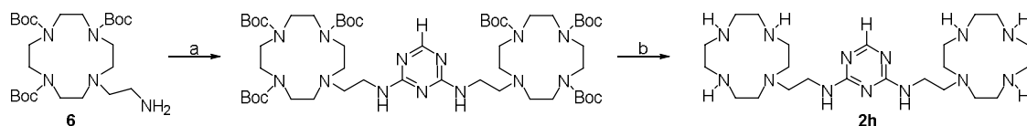
Scheme 3 Preparation of the cleaving agent 2h . Reagents and conditions: (a) 2,4-dichlorotriazine, DIPEA, MeCN, (b) TFA, CH 2 Cl 2 , MeOH.
