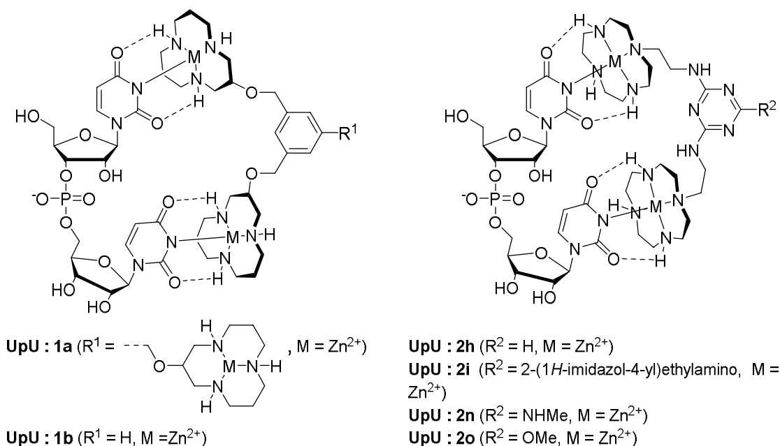
Fig. 1 Complexes of UpU with bi- and trinuclear \text{Zn}^{\text{II}} chelates of 1,5,9-triazacyclododecane ( 1a and 1b ) and cyclen ( 2h , 2i , 2n and 2o ).
