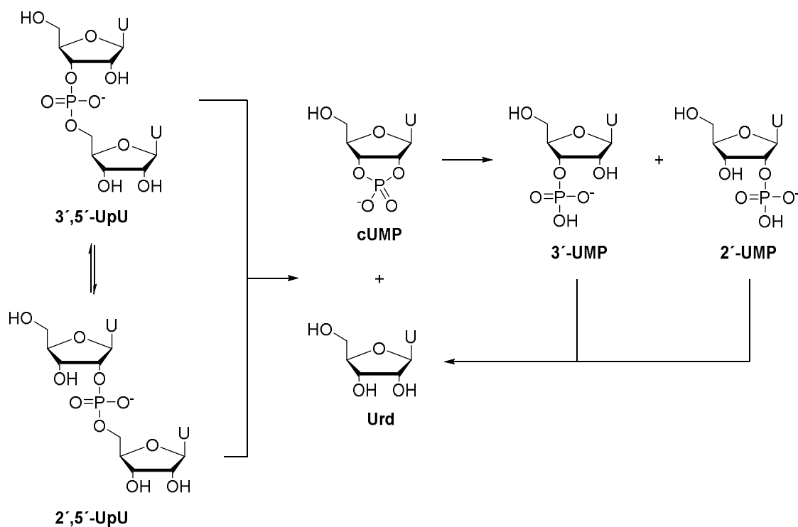
Scheme 5 Hydrolytic reaction pathways of UpU.
