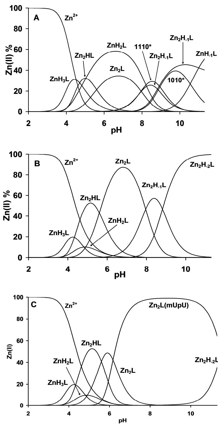
Fig. 2 Species distribution curves for the Zn^{II} complexes in the Zn^{II} / L / mUpU = 1/1/0 (A), 2/1/0 (B) and 2/1/1 (C) systems ( T = 25\text{ }^{\circ}C , I(\text{NaCl}) = 0.1\text{ mol L}^{-1} , [L] = 1\text{ mmol L}^{-1} ).
