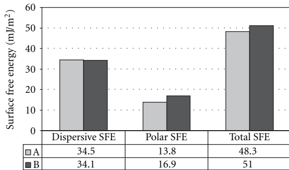
FIGURE 5: Dispersive ( \gamma^D ), polar ( \gamma^P ), and total ( \gamma^{TOT} ) components of surface free energy (SFE) calculated using the Owens-Wendt approach: (A) in-plane distribution of fibers; (B) transverse distribution of fibers.
