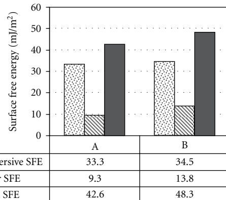
FIGURE 6: Dispersive ( \gamma^D ), polar ( \gamma^P ), and total ( \gamma^{TOT} ) components of surface free energy (FRC) calculated using the Owens-Wendt approach: (A) fibers running in-plane (perpendicular) to the camera axis; (B) fibers running in-plane (parallel) to the camera axis.
