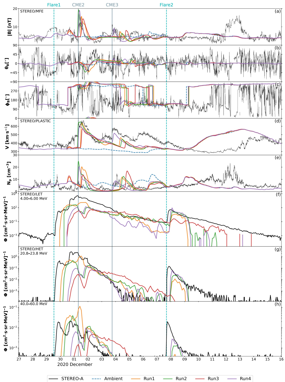
Figure A2. WSA-Enlil-SEPMOD results at Solar Terrestrial Relations Observatory-Ahead (STEREO-A) shown against STEREO-A data. The parameters shown are: (a) magnetic field magnitude, (b) \theta and (c) \phi angles of the magnetic field, (d) solar wind speed, (e) proton density, and (f–h) particle measurements in three different energy channels.
