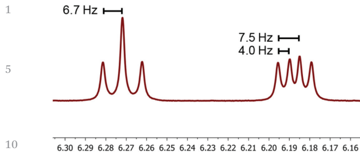
Fig. 3 The signals corresponding to the C1' protons in TnpsT 1 . The signal at 6.27 ppm corresponds to the 5'-linked nucleoside ( psT ), while the signal at 6.19 ppm corresponds to the 3'-linked nucleoside ( Tnp ).
