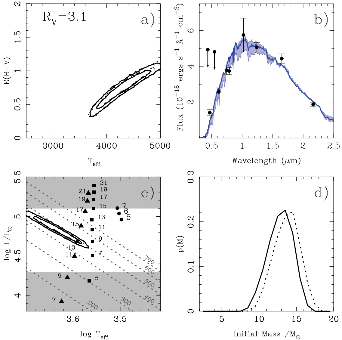
Figure 6. The derived properties of the progenitor of SN 2008bk, assuming R_V = 3.1 for \log(Z/Z_{\odot}) = -0.25 and 0.0 . (a) The joint posterior distribution for reddening E(B - V) and temperature T_{\text{eff}} . The solid and dashed contours correspond to metallicities of \log(Z/Z_{\odot}) = -0.25 and 0.0 , respectively. The contours contain 68 and 95 per cent of the probability for each model fit. (b) The observed photometry, and detection limits, of the progenitor compared to the best-fitting SED model (heavy line). The shaded SED envelope corresponds to the 68 per cent probability interval. (c) The position of the progenitor on the HR diagram. The meaning of the contours is the same as above. The shaded regions indicate locations on the HR diagram that are inconsistent with the measured K_S -band brightness. Overplotted are the points from LMC metallicity STARS stellar evolution models, with initial masses as labelled, corresponding to the positions of the end of He-burning ( \blacktriangle ), the termination point of the models ( \blacksquare ) and the termination point for those stars that become SAGB stars ( \bullet ). The dashed grey lines show lines of constant radius on the HR diagram. (d) Mass probability density distributions for the progenitor of SN 2008bk, for \log(Z/Z_{\odot}) = -0.25 (solid) and 0.0 (dashed).
