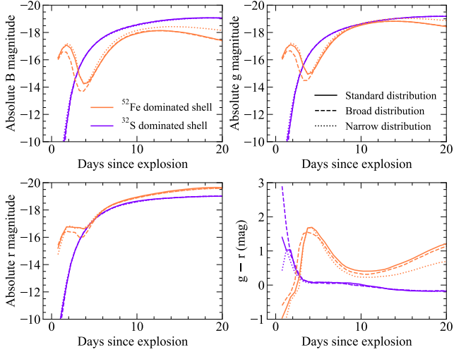
Figure C1. Light curves and colours for models with different shell isotope distributions. All models shown have a 1.0 M_{\odot} core and a 0.04 M_{\odot} shell, of which 50% is burned to elements heavier than helium. We show models with dominant shell products of ^{52}\text{Fe} and ^{32}\text{S} , as representative of models with IGE- and IME-dominated shells.
