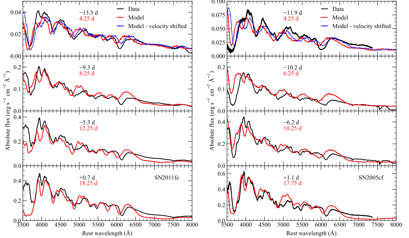
Figure 13. Comparisons between spectra of SNe 2011fe and 2005cf (black), and our double-detonation models with ^{32}\text{S} -dominated shells (red) at epochs from 4 – 18 d after explosion, along with the parameters of both models. Spectra are shown on an absolute flux scale. For the first epoch, we also show model spectra shifted in velocity to provide better agreement to the observed features (blue). The phases of the observed spectra of SNe 2011fe and 2005cf relative to B -band maximum are given in black, while the time since explosion for our model comparison spectra is shown in red.
