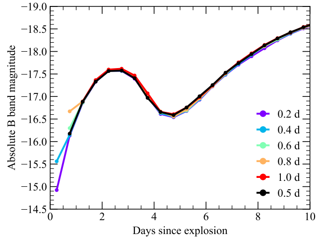
Figure A1. Light curves calculated with different simulation start times for an ^{52}\text{Fe} -dominated shell. Our nominal start time of 0.5 d after explosion is shown in black.
