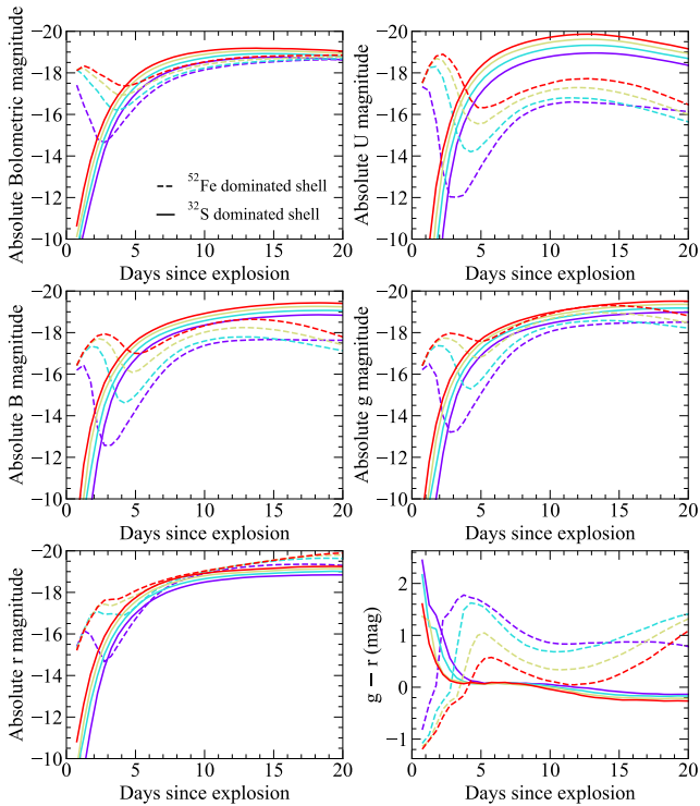
Figure 8. Light curves and colours for models with different shell masses. All models shown have a 1.0 M_{\odot} core and we assume 80% of the shell is burned to elements heavier than helium. We show two representative cases in which the composition of the shell is dominated by either ^{32}\text{S} or ^{52}\text{Fe} .
