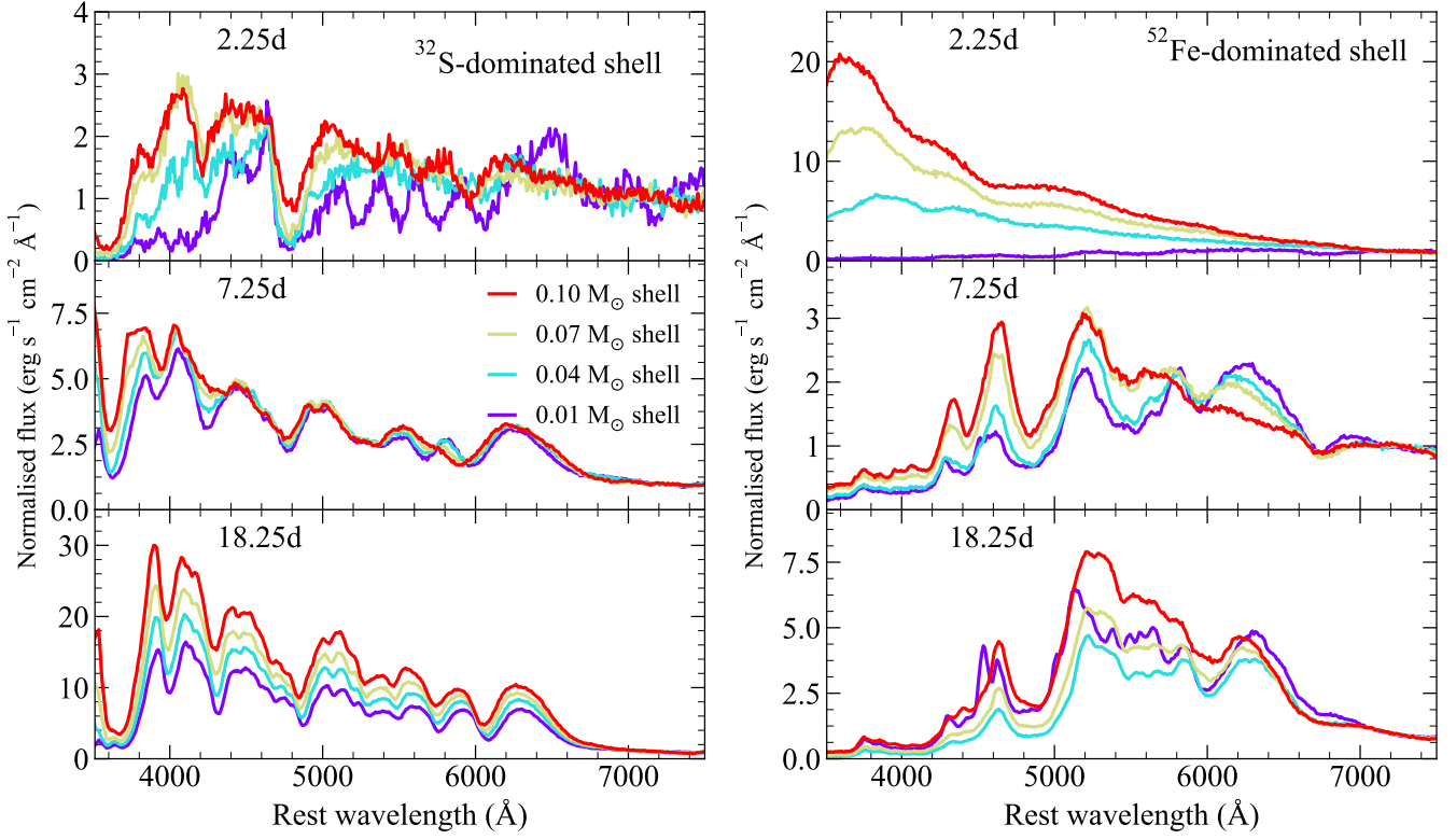
Figure 9. Spectra for models with different shell masses. All models shown have a 1.0 M_{\odot} core and we assume 80% of the shell is burned to elements heavier than helium. We show two representative cases in which the composition of the shell is dominated by either ^{32}\text{S} or ^{52}\text{Fe} . Spectra are shown at three epochs: 2.25 d, 7.25 d, 18.25 d after explosion. All spectra are normalised to the flux between 7000 – 7500 Å.
