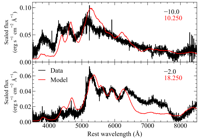
Figure 18. Comparison between spectra of SN 2018byg (black) and our model with a 0.9 M_{\odot} core and 0.1 M_{\odot} shell (red). Phases of SN 2018byg are given relative to r -band maximum, while days since explosion are given for our model. Spectra are shown in scaled flux.
