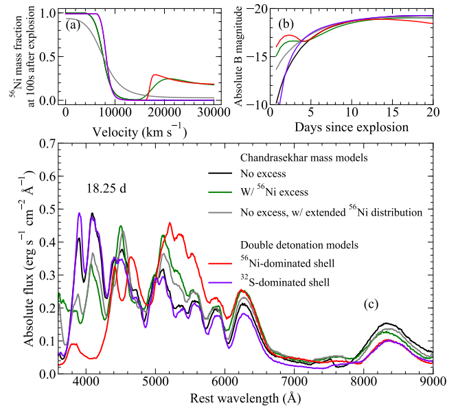
Figure 11. Panel a: Comparison between the ^{56}\text{Ni} distributions for models presented here. We show a Chandrasekhar mass model from Magee & Maguire (2020) that contains a ^{56}\text{Ni} excess in the outer ejecta and the corresponding model without an excess, in addition to a model with an extended ^{56}\text{Ni} distribution. Double detonation models with a ^{56}\text{Ni} - and ^{32}\text{S} -dominated shell (red and purple, respectively) are also shown. Panel b: B -band light curve for models presented here. Panel c: Comparison of spectra for our models at 18.25 d after explosion.
