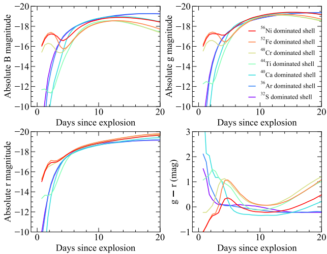
Figure 5. Light curves and colours for models with different shell compositions. All models shown have a 1.0 M_{\odot} core and a 0.07 M_{\odot} shell, of which 50% is burned to elements heavier than helium. The dominant \alpha -chain product produced in the shell is given by the colours. The relative fractions of all other isotopes in the shell are given following from Fig. 4.
