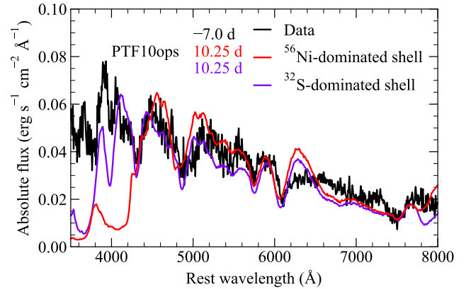
Figure 20. Comparison between the spectrum of PTF10ops approximately one week before B -band maximum (black) and our models with a 0.9 M_{\odot} core, 0.01 M_{\odot} shell and either a ^{56}\text{Ni} -dominated (red) or ^{32}\text{S} -dominated (purple) composition for the shell. Phases for the model spectra are given as days since explosion. All spectra are shown in an absolute flux scale.
