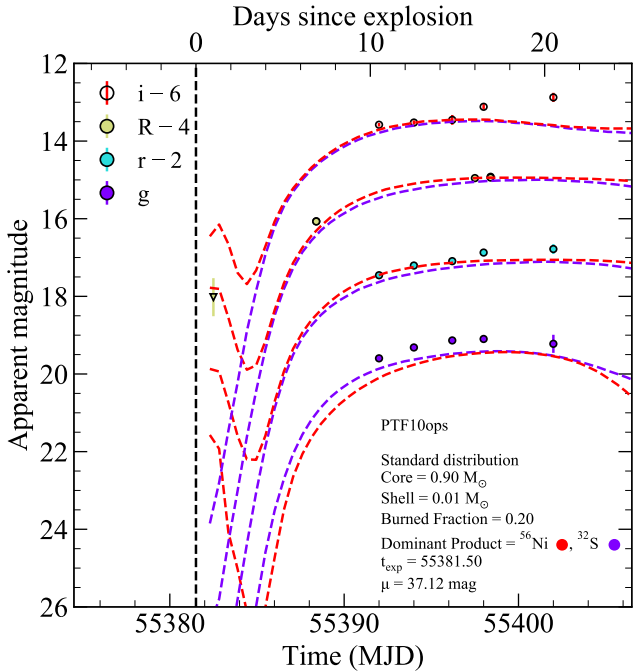
Figure 19. Comparison between the light curve of PTF10ops and our models with a 0.9 M_{\odot} core, 0.01 M_{\odot} shell and either a ^{56}\text{Ni} -dominated (red) or ^{32}\text{S} -dominated (purple) composition for the shell. The explosion epoch is shown as a vertical dashed line.
