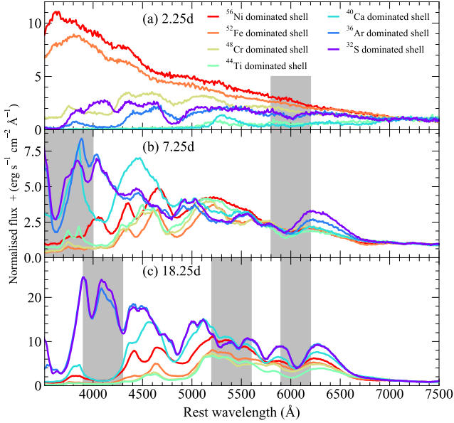
Figure 6. Spectra for models with different shell compositions. All models shown have a 1.0 M_{\odot} core and a 0.07 M_{\odot} shell, of which 50% is burned to elements heavier than helium. The dominant \alpha -chain product produced in the shell is given by the colours. The relative fractions of all other isotopes in the shell are given following from Fig. 4. Spectra are shown at three epochs: 2.25 d, 7.25 d, and 18.25 d after explosion. All spectra are normalised to the flux between 7000 - 7500 \text{ \AA} . Features discussed in the main text are shown as shaded regions.
