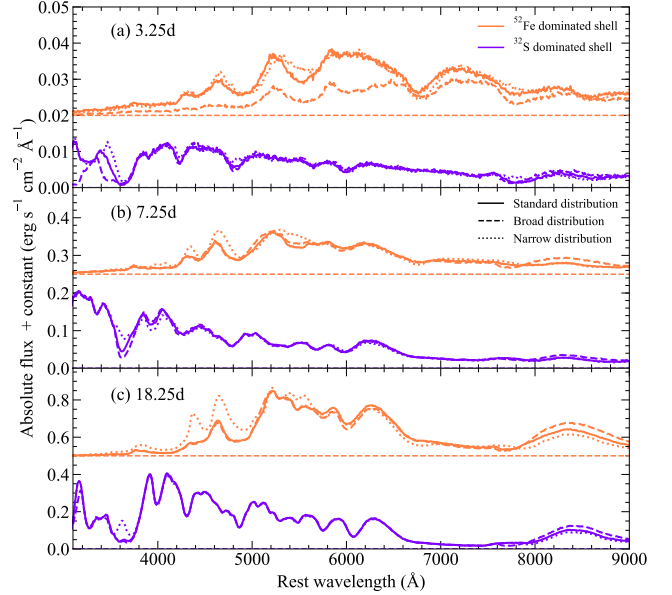
Figure C2. Spectra for models with different shell isotope distributions. All models shown have a 1.0 M_{\odot} core and a 0.04 M_{\odot} shell, of which 50% is burned to elements heavier than helium. We show models with dominant shell products of ^{52}\text{Fe} and ^{32}\text{S} , as representative of models with IGE- and IME-dominated shells. Spectra are shown at three epochs relative to explosion: 3.25 d, 7.25 d, and 18.25 d.
