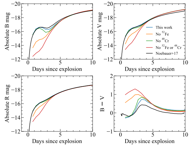
Figure 1. Comparison between the sub-Chandrasekhar mass double detonation model calculated by Noebauer et al. (2017) using STELLA (black) and our calculation using TURTLS (blue).
