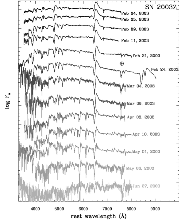
Figure 13. Spectral evolution of SN 2003Z. Symbol ⊕ indicates telluric absorptions.
