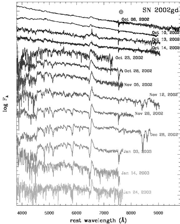
Figure 12. Sequence of spectra of SN 2002gd during the photospheric phase. Symbol ⊕ indicates telluric absorptions.
