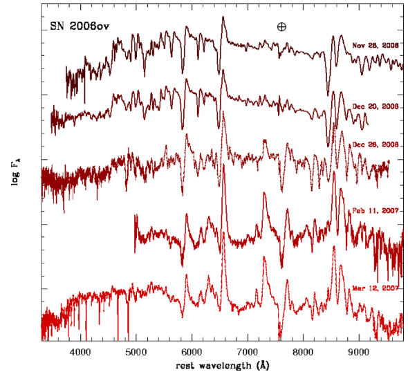
Figure 14. Sequence of spectra of SN 2006ov from photospheric to nebular phase. Significant contamination from the background explains the blue excess at late phase. Symbol ⊕ indicates telluric absorptions.
