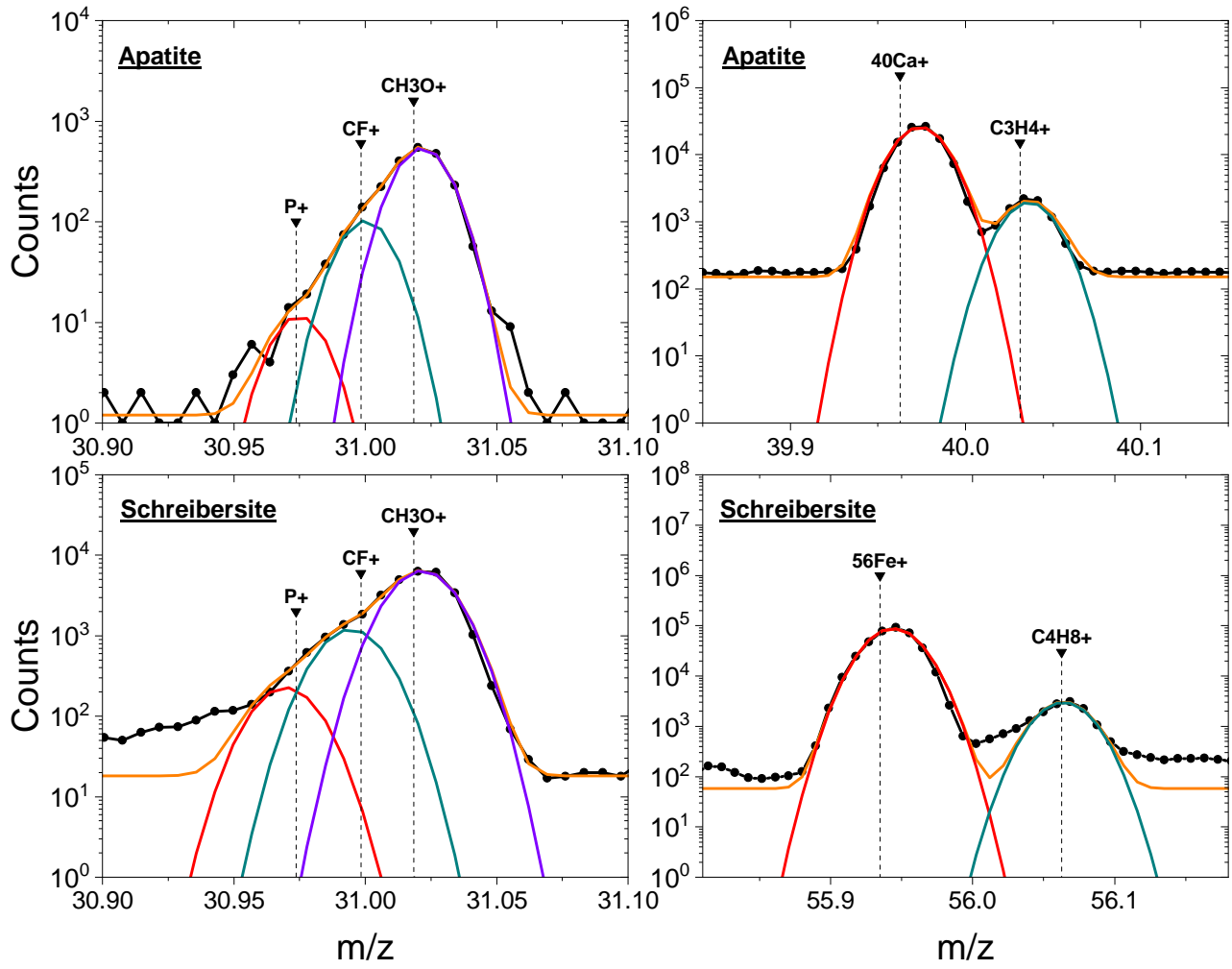
Figure 2. Positive spectra for the reference materials measured on Earth on the reference COSIMA instrument, showing the presence of phosphorus as well as the main positive peak present in the substance. The mass calibration for Apatite is off at higher masses due to the methodology not being perfect for pure reference material. Notice the multiple orders of magnitude that separate the signal of Fe/Ca in comparison to P.
