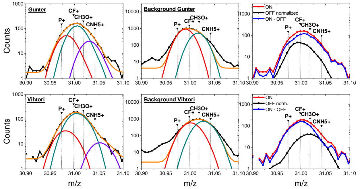
Figure 1. As Fig 1 for particles Vihtori and Günter.
