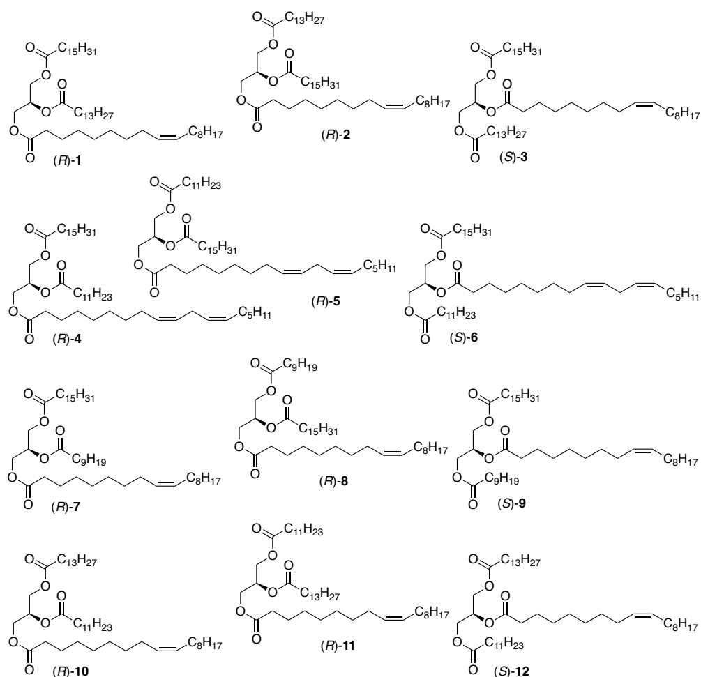
Figure 1. The structures of the twelve enantiostructured TAG products synthesised.
