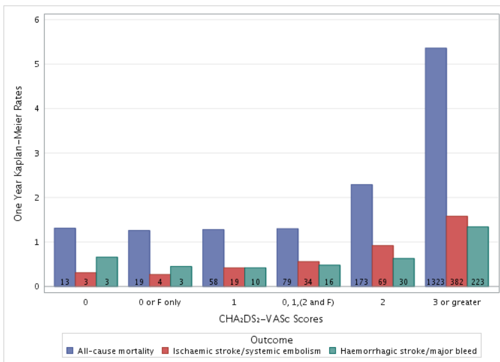
Figure 1 One-year Kaplan-Meier event rates by CHA 2 DS 2 -VASc score for all-cause mortality, ischaemic stroke/systemic embolism and haemorrhagic stroke/major bleed. F, female.
