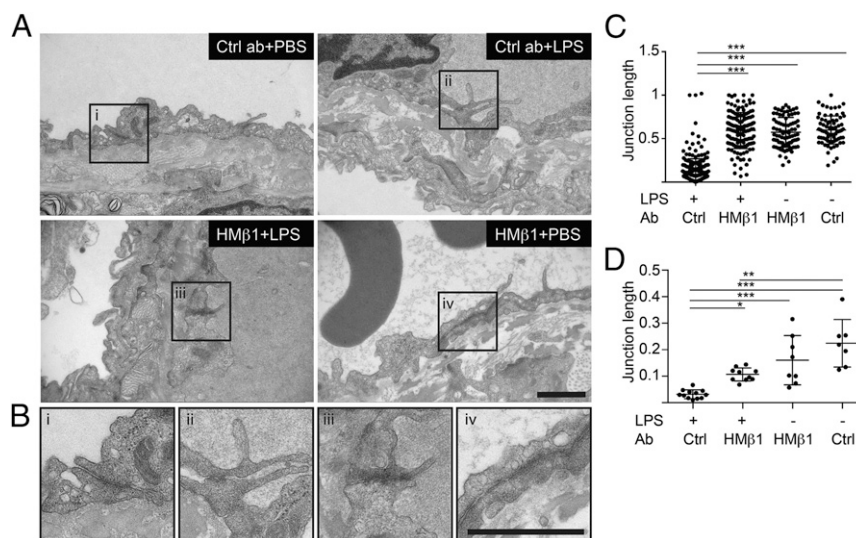
Fig. 5. \beta 1-integrin antibody improves endothelial cell junction integrity in endotoxemia. LPS or PBS was administered to mice 24 h after the administration of HMP \beta 1 or control antibody. (A) Representative transmission electron microscopic images of lungs 16 h after LPS or PBS administration. (B) Magnification of the area indicated in A. (C and D) Quantification of the electron-dense areas of endothelial cell–cell junctions relative to total endothelial cell–cell contact in the lungs (C) and (D) trachea, as described in more detail in SI Appendix, SI Materials and Methods and Fig. S14 . Data are the mean \pm SD of n = 3 mice per group. * P < 0.05 , ** P < 0.01 , and *** P < 0.001 (Tukey's test). (Scale bars: 1 \mu m).
