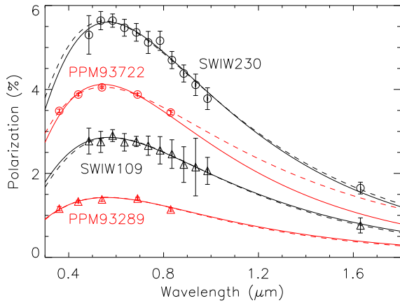
Figure 3. Example fits to the Serkowski curve for four stars. Black circles and triangles represent data for two high-extinction stars at 11 optical wavelength bins and H -band, while the red points represent low-extinction stars at the UBVRI passbands only. Solid lines represent fits to the Serkowski relation (with parameter K = 1.15 ) whereas K is allowed to float in the dashed-line fits to the Wilking relation.
