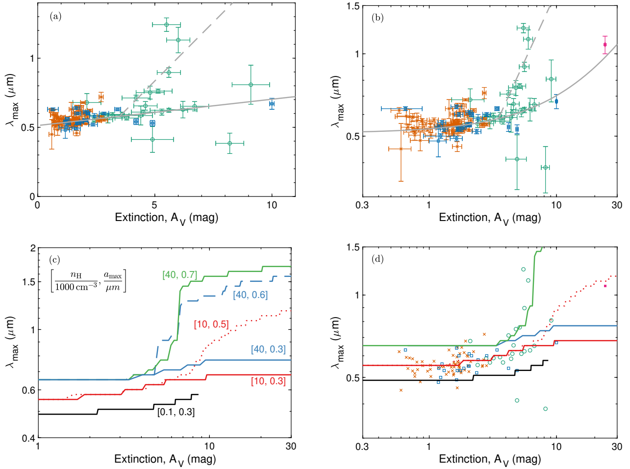
Figure 5. Panels (a) and (b) show the relation between the wavelength peak of the polarization curve ( \lambda_{\max} ; equation [1]) and optical extinction ( A_V ) towards stars behind Taurus. Data are from both this work (Kast/Lick = green and TurPol/NOT = orange) and Whittet et al. (2001; blue). Panel (a) is plotted using linear axes while panel (b) is plotted logarithmically and also includes the data point for Elias 3-16 (Hough et al. 1988; Murakawa et al. 2000; magenta). The solid and dashed lines show the best linear fits to the “upper” and “lower” branches (Table 7), respectively. (c) Model fits based on RAT alignment are shown for a number of model parameters. Lines are labeled with the volume density (in units of 1000 \text{ cm}^{-3} ) and the maximum grain size ( \mu\text{m} ) in each model. In order to show the key model differences, the plot shows a slightly different range of A_V and \lambda_{\max} from panels a, b, and d. Panel (d) compares several of the models in panel c (using the same color scheme) with the data in panels a and b. The error bars on the data are removed for clarity only.
