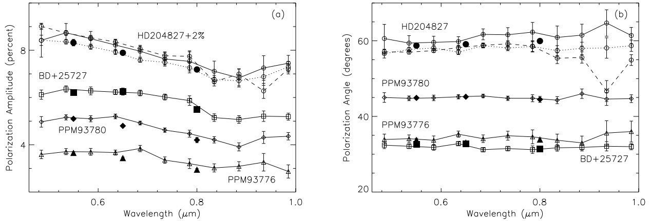
Figure 7. Polarization amplitudes (a) and angles (b) measured for standard high-polarization stars (see Table 9). All three separate measurements for HD 204827 are shown as open circles with different observations indicated by different line-types. Error-bars represent only the statistical uncertainties in the polarization fits and do not include any estimate of systematic uncertainties. Large solid symbols show TurPol measurements of all four stars through broadband V ( 0.55 \mu\text{m} ), R ( 0.65 \mu\text{m} ), and I ( 0.80 \mu\text{m} ) filters (see text for references and band definitions). Uncertainties for data without error-bars are smaller than the plotted symbols. For clarity, the polarization amplitude data for HD 204827 have been shifted up by 2%.
