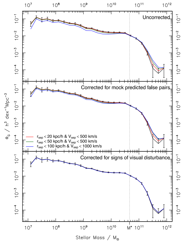
Figure 18. Depiction of the effect on the GSMF presented in Baldry et al. (2012) if the different close pair selections shown in Fig. 16 were assumed to merge on some unknown time-scale. The top panel is only corrected for galaxies appearing in multiple close pairs. The middle panel is true pair corrected from the mock catalogues using W_{TP-mock} (see Section 3.4). The bottom panel is corrected for the fraction of visually disturbed galaxies in pairs using W_{TP-vc} (see Section 3.4). In all cases mass is moved from moderate stellar mass galaxies ( 10^8 – 10^{10} M_\odot ) to beyond \mathcal{M}^* (although this is hard to identify in the bottom panel). This has the inevitable effect of enhancing the dip in this regime, increasing the significance of the double-Schechter shape in the GSMF and moving the future value of the GSMF \mathcal{M}^* to larger masses.
