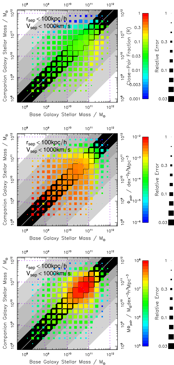
Figure 9. Pair properties for r_{\text{sep}} < 100 \text{ kpc} and v_{\text{sep}} < 1000 \text{ km s}^{-1} sample ( PS_{r20v1000} true pair corrected using the mock catalogues ( W_{\text{TP-mock}} , see Section 3.4). For more information see the caption for Fig. 7.
