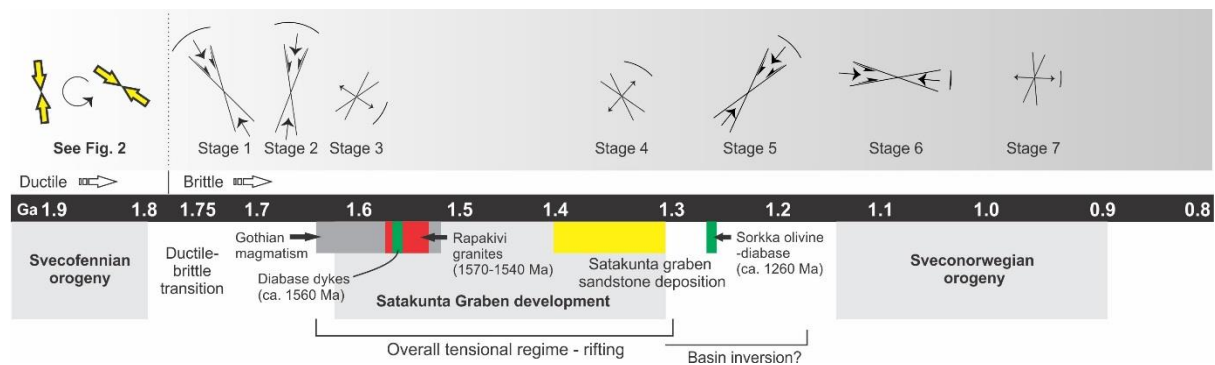
Fig. 3. Summary of major crustal events from 1.9 to 0.8 Ga (bottom) and conceptual model over the brittle evolution of southwestern Finland (top; modified after Mattila and Viola, 2014). The filled yellow arrows refer to the palaeostress configurations of the ductile evolution pre-dating the brittle deformation.
