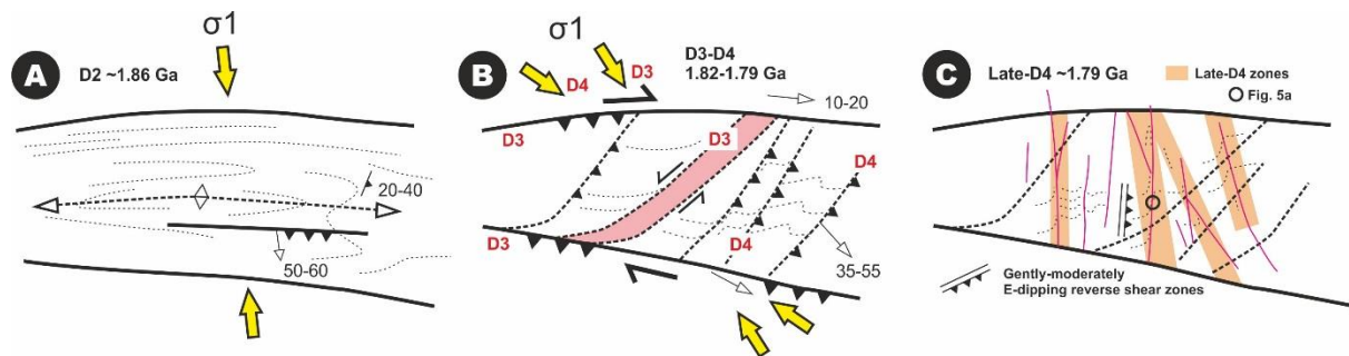
Fig. 2. Schematic representation of the tectonic evolution of the Olkiluoto area. A: D2-stage characterised by N-S compression and development of dominantly E-plunging upright folds. B: D3-D4 -stage characterised by dextral reverse shearing along E-W shear zones, development of NE-SW to NNE-SSW striking, gently to moderately dipping reverse shear zones under NW-SE to WNW-ESE compression (D3 and D4, respectively). C: Development of late-D4 zones of incomplete structural transposition along pre-existing crustal discontinuities, as a progression of the D4-stage, and schematic illustration over their relationship with the approximately N-S striking brittle fault zones (purple).
