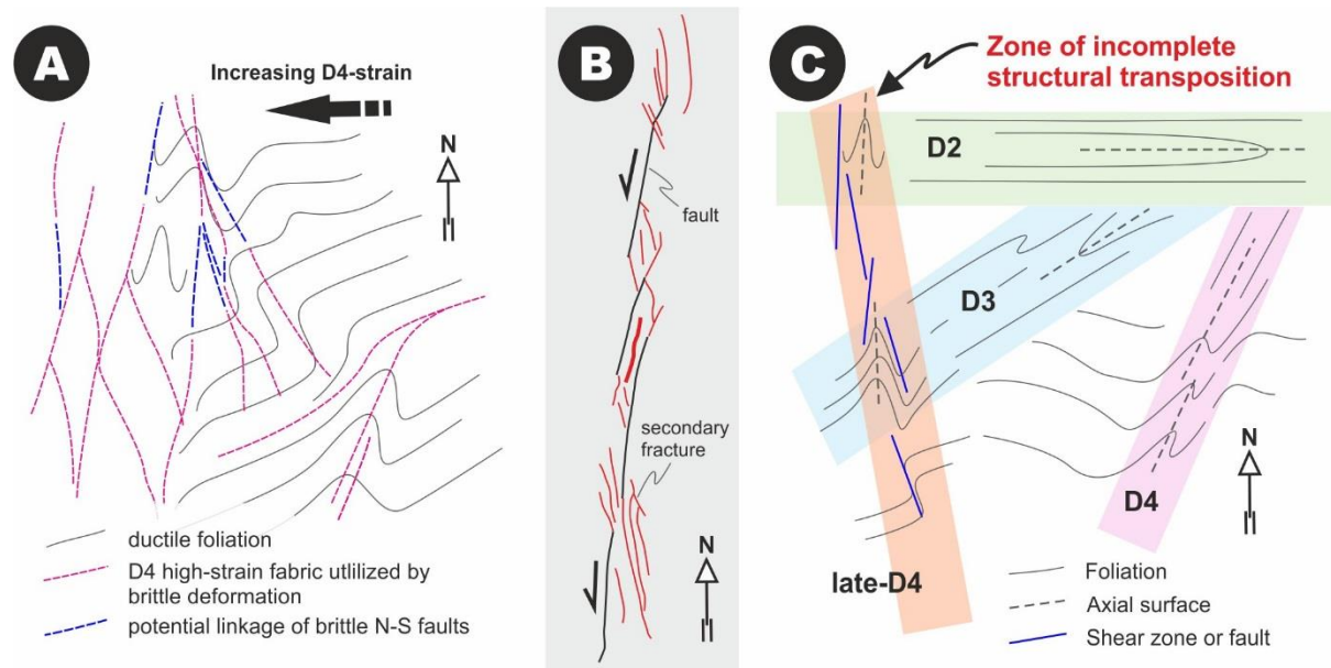
Fig. 6: A conceptual model explaining the origin of the N-S faults in Olkiluoto. A: Development of (late-) D4 high strain fabrics along the short limbs of F4 folds and formation of anastomosing shear zone networks. B: Conceptual model of fracture linkage from en échelon set of joints (after Joussineau et al., 2007). C: Structural zones with either complete or high degree of transposition (D2-4), characterised by structural elements parallel to the zone orientation, and the introduced zone of incomplete structural transposition (late-D4), characterised by structural elements at oblique angles to, but preferential occurrence within the zone.
