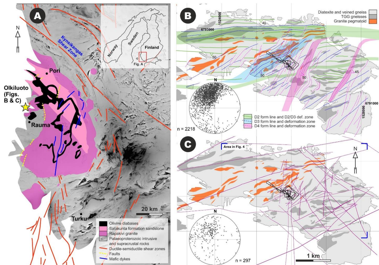
Fig. 1. A: Geological setting of Olkiluoto after Korsman et al. (1997). Aeromagnetic map by Geological Survey of Finland. B: The ductile structural framework of Olkiluoto. The equal-area, lower hemisphere projections show the orientation distribution of all the ductile foliations measured from the ground surface. C: Surface intersections of the modelled Brittle Fault Zones (BFZ). The equal-area, lower hemisphere projections show the orientation all the modelled BFZ surfaces. B and C: Data from Aaltonen et al. (2016). The black line is the
