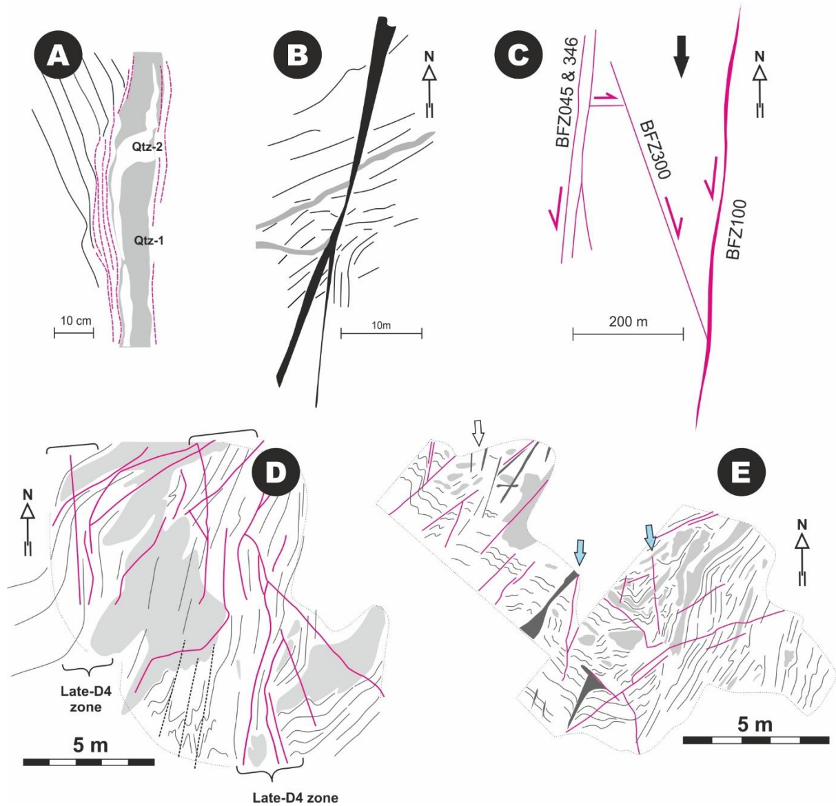
Fig. 5. A: Deflection of the host-rock foliation (black lines) into the shear zone precursor (magenta lines) of the brittle fault zone BFZ-045. Redrawn after Mattila (2009). B: Main foliation (black lines) deflection associated with the brittle fault zone BFZ-100 (black polygons) and the older ductile shear zones (grey polygons; redrawn after Mattila et al., (2007 [TK-11]). C: Geometric and kinematic summary of the network of approximately N-S striking brittle deformation zones at disposal level in Olkiluoto, including the dominant sinistral and the secondary dextral zones (BFZ-300). Sketch map from -420 m level after Aaltonen et al., 2016. D: Development of N-S striking fracture arrays along the short limbs of D4 folds. Black and purple lines represent ductile and
