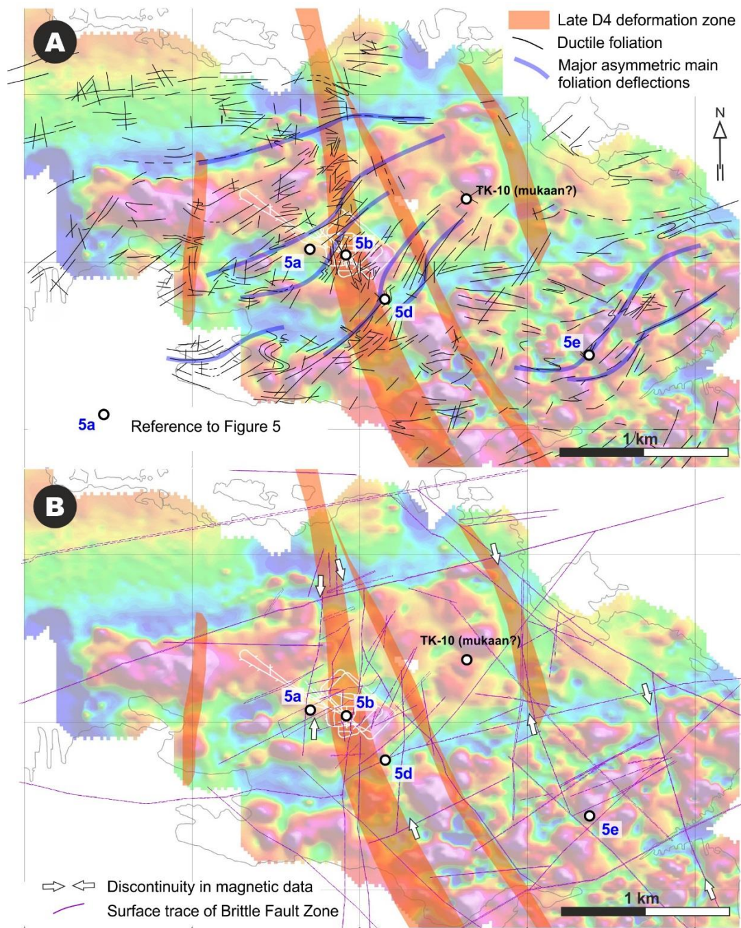
Fig. 4. A: A revised structural interpretation with foliation form lines and late-D4 deformation zones. The interpretation is based on a total of 2218 foliation measurements from the ground surface (Fig. 1b), complemented by 132 foliation strike readings with no dip data. The ground magnetic map is from Posiva, white line is the surface projection of ONKALO (see Fig. 1 caption). B: Correlation of the late-D4 deformation zones and the brittle fault zone intersections at ground surface level. The white arrows exemplify the locations of N-S
