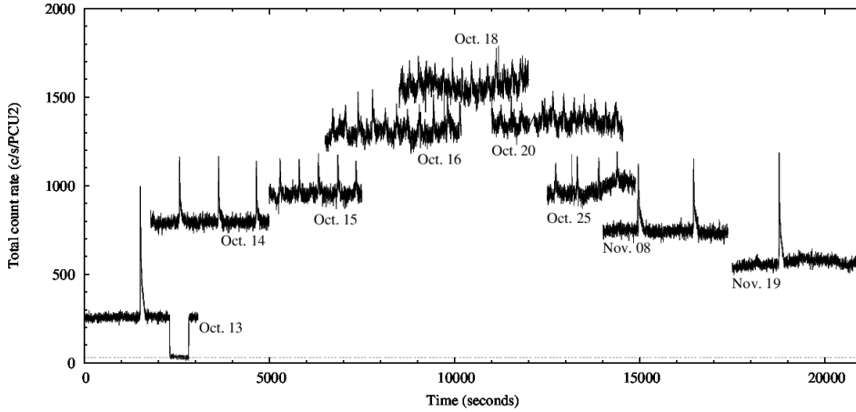
Figure 8: The evolution of the thermonuclear burst frequency in IGR J17480-2446 during the course of its 2010 outburst. Data were obtained from RXTE and the x-axis shows the time at different phases of the outburst, which evolution of the persistent emission is represented in the y-axis in units of count-rate recorded by the PCU2 on-board RXTE . Times have been shifted arbitrarily for display purposes. Credit: Linares et al., ApJ , 748, 2 (2012). reproduced with permission of the AAS.
