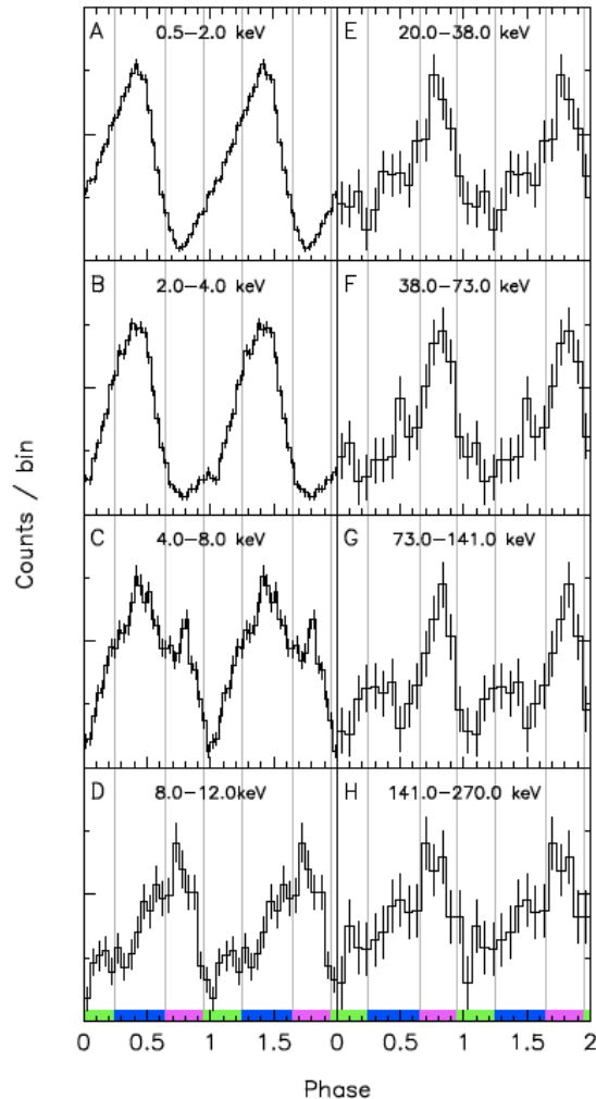
Figure 17: Pulse profiles of 1RXS 1708–4009 (from (den Hartog et al., 2008a)) obtained in the soft X-ray band with XMM-Newton (left panels) and in the hard X-ray band with INTEGRAL (right panels). Observations were not strictly simultaneous. Credit: den Hartog et al., A&A, 489, 263 (2008), reproduced with permission (ESO).
