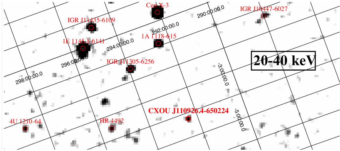
Figure 12: Top panel: Chandra /ACIS-I 0.3–8 keV image of the field around CXOU J110926.4–650224 with the error circles of the counterparts from INTEGRAL (IGR J11098–6457, 20–40 keV, magenta line) Swift /BAT (4PBC J1109.3–6501, 15–150 keV, yellow line) and Fermi /LAT (FL8Y J1109.8–6500, 100 MeV–300 GeV, green line) catalogues. Bottom panel: INTEGRAL IBIS/ISGRI 20–40 keV mosaic image of the field around IGR J11098–6457. Credit: Coti Zelati et al., A&A , 622, A211 (2019), reproduced with permission (ESO).
