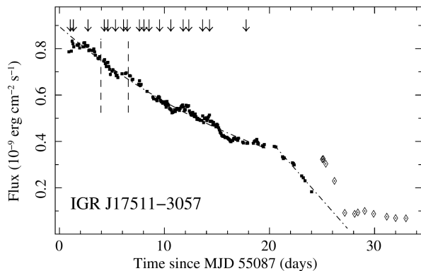
Figure 2: The light curve of the outburst of IGR J17511-3057 observed in 2009 (Falanga et al., 2011). The typical exponential decay profile is clearly visible, with a break occurring about 20 days after the onset of the event. The light curve is obtained from the RXTE /PCA (2–20 keV) data, with the vertical dashed lines indicating the interval of the INTEGRAL observations. The arrows mark the times of the detected X-ray bursts. The diamonds refer to the observations in which both IGR J17511-3057 and XTE J1751-305 were active and the instruments on-board RXTE were unable to separate the contribution of the two sources. Credit: Falanga et al., A&A , 529, A68 (2011), reproduced with permission (ESO).
