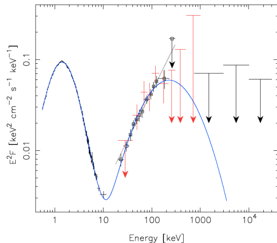
Figure 16: The broad band spectrum of 4U 0142+61 (from den Hartog et al., 2008b)). The data below 10 keV are from XMM-Newton , while those above 20 keV are from the INTEGRAL IBIS/ISGRI (black) and SPI (red) instruments. The upper limits in the 0.75–30 MeV range are from COMPTEL. The blue line is a best fit with a phenomenological model consisting of the sum of log-parabolic functions, that clearly illustrates the different components at soft and hard X-ray energies. Credit: den Hartog et al., A&A, 489, 245 (2008), reproduced with permission (ESO).
