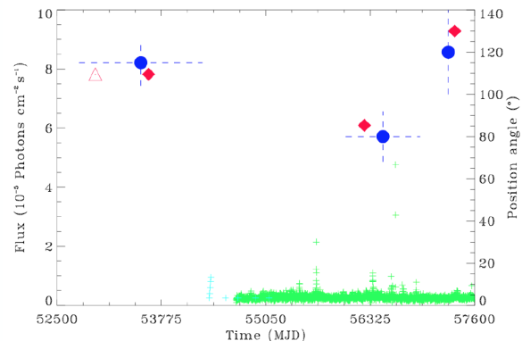
Figure 13: Galway Astronomical Stokes Polarimeter (GASP, Collins et al. 2013, open triangle and filled diamonds) and INTEGRAL observations of the polarisation position angle of the Crab (blue filled circles; Moran et al. 2016; O'Connor et al. 2018). Green and cyan points show the flux observed by Fermi and AGILE , respectively. More recent Astrosat measurements (Vadawale et al., 2018) in the 0.1-0.38 MeV band indicate a polarisation angle of (143.5 \pm 2.8)^\circ consistent with the trend observed by GASP and INTEGRAL . Credit: Moran et al., MNRAS, 456, 2974 (2016), reproduced with permission of Oxford University Press on behalf of the Royal Astronomical Society.
