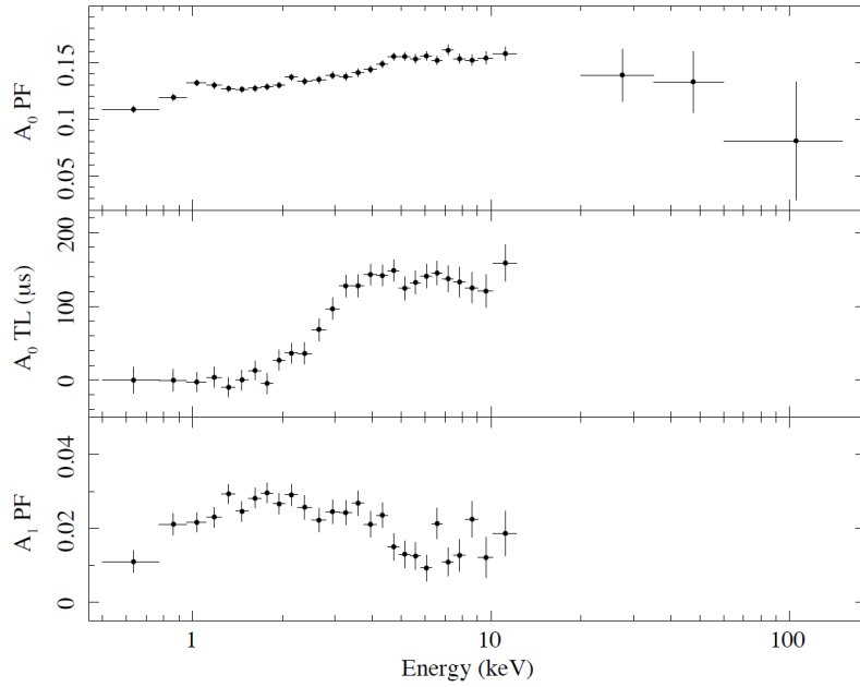
Figure 11: Top panel: pulse profiles of IGR J18245–2452 observed by XMM-Newton /EPIC-pn (panels a-f), INTEGRAL IBIS/ISGRI (panels g-i) and Fermi /GBM (panel j); bottom panel, from top to bottom: pulsed fraction of the first harmonic, hard phase/time lags, and pulsed fraction of the second harmonic. Credit: De Falco et al., A&A , 603, A17 (2017), reproduced with permission (ESO).
