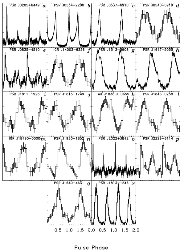
Figure 14: The pulse shapes of all soft \gamma -ray pulsars in the catalog (Kuiper and Hermsen, 2015). The profiles are measured either with INTEGRAL IBIS/ISGRI or RXTE PCA or HEXTE. Exceptions are PSR J1640-4631 ( NuSTAR ) and PSR J1813-1246 ( XMM-Newton EPIC). Credit: Kuiper & Hermsen, MNRAS, 449, 3827 (2015), reproduced with permission of Oxford University Press on behalf of the Royal Astronomical Society.
