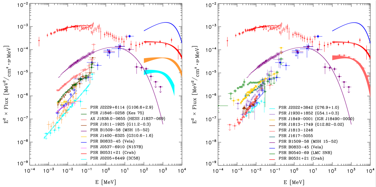
Figure 15: The high-energy pulsed emission spectra for 17 of the 18 detected soft \gamma -ray pulsars from 0.1 keV – 10 GeV summarized in two panels. The spectra of PSR B0531+21 (Crab), PSR B0833-45 (Vela) and PSR B1509-58 are shown in both panels for reference purposes. The pulsed spectrum of PSR J1640-4631 is not shown, because its total spectrum has been reported up to hard X-rays but its pulsed spectrum just up to 25 keV. Credit: Kuiper & Hermsen, MNRAS, 449, 3827 (2015), reproduced with permission of Oxford University Press on behalf of the Royal Astronomical Society).
