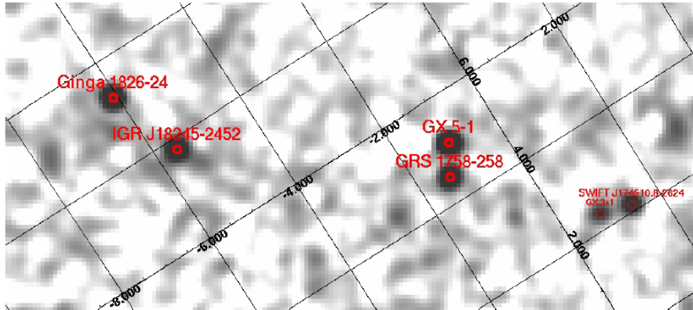
Figure 9: Mosaic of the IBIS/ISGRI field around IGR J18245-2452 at the time of its discovery in 2013 (Papitto et al., 2013).
