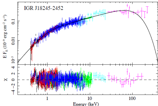
Figure 10: The unfolded absorbed broad-band spectrum of IGR J18245–2452 observed during the 2013 X-ray outburst, fitted with a Comptonization compss model (black line). Data points from XMM-Newton /RGS (red and black points, 0.4–1.8 keV), XMM-Newton /EPIC-pn (green points, 0.9–11 keV), Swift /XRT (blue points, 0.4–8 keV), INTEGRAL /JEM-X (light blue points, 5–25 keV) and INTEGRAL IBIS/ISGRI (magenta points, 22–250 keV) were included. The bottom panel shows residuals with respect to the best fit model. Credit: De Falco et al., A&A , 603, A17 (2017), reproduced with permission (ESO).
