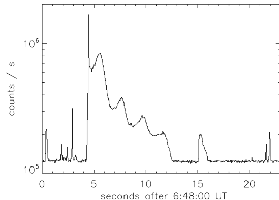
Figure 18: The SPI/ACS light curve at E > 80 keV of a bright burst observed from 1E 1547.0–5408 on January 22, 2009. The tail following the bright initial pulse clearly shows the NS rotation period of 2.1 s. Credit: Mereghetti et al., ApJ, 696, L74 (2009), reproduced with permission of the AAS.
