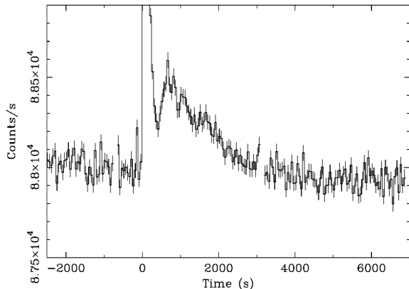
Figure 19: SPI/ACS light curve ( E > 80 keV) of the December 27, 2004 giant flare from SGR 1806–20 (from Mereghetti et al. 2005b). Due to the rebinning at 50 s, the 7.6 s pulsations in the tail time interval (1–400 s) are not visible in this figure. After the pulsating tail, the flux increases again, peaking \sim 700 s after the beginning of the flare and decreasing below the background level about one hour later. Note that the peak of the flare at t = 0 , reaching an observed count rate > 2 \times 10^6 counts s^{-1} , is out of the vertical scale. Credit: Mereghetti et al., ApJ, 624, L105 (2005), reproduced with permission of the AAS.
