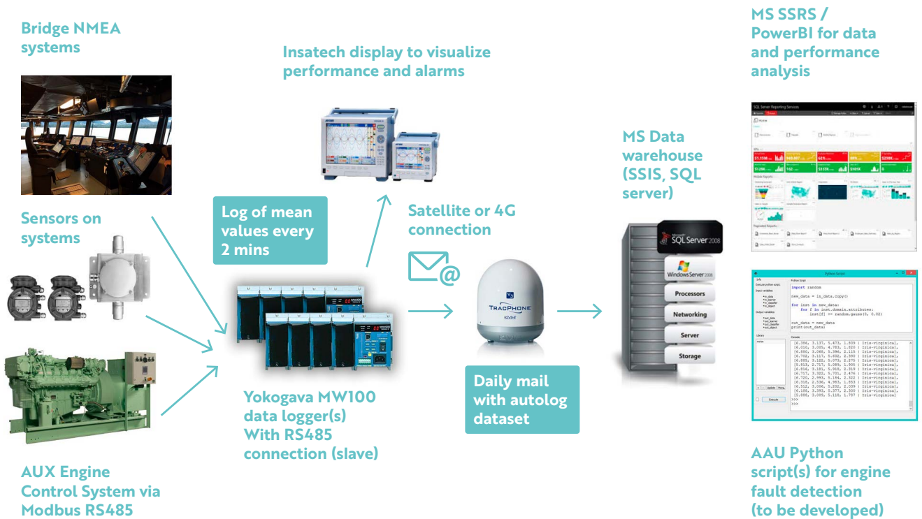
FIGURE 7. ILLUSTRATION OF LAURITZEN DATA VALUE CHAIN AND VESSEL PERFORMANCE MONITORING SET-UP FOR AUTOLOG DATA
