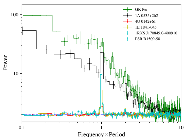
Fig. 1. Power density spectra of the magnetized compact objects discussed in the text and labeled in the legend. The frequency is expressed in units of respective objects spin frequency and power is normalized such that expected white noise level is 2.
