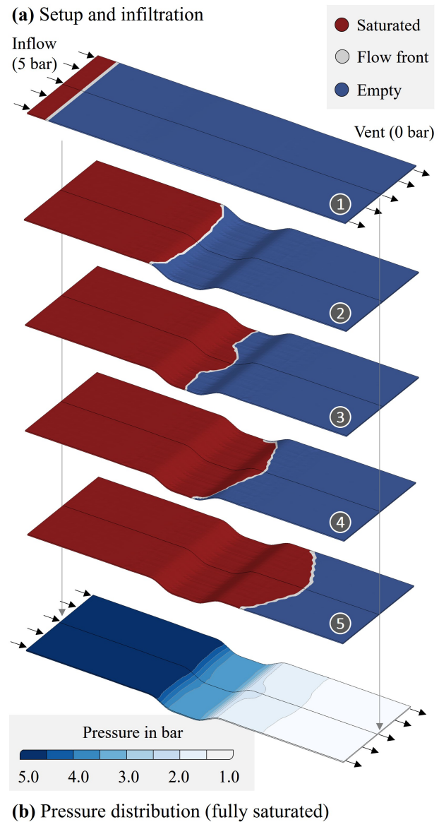
Fig. 9: Simultaneous infiltration of the hybrid stack; (a) Flow front progression; (b) Final pressure distribution for the fully saturated specimen.
