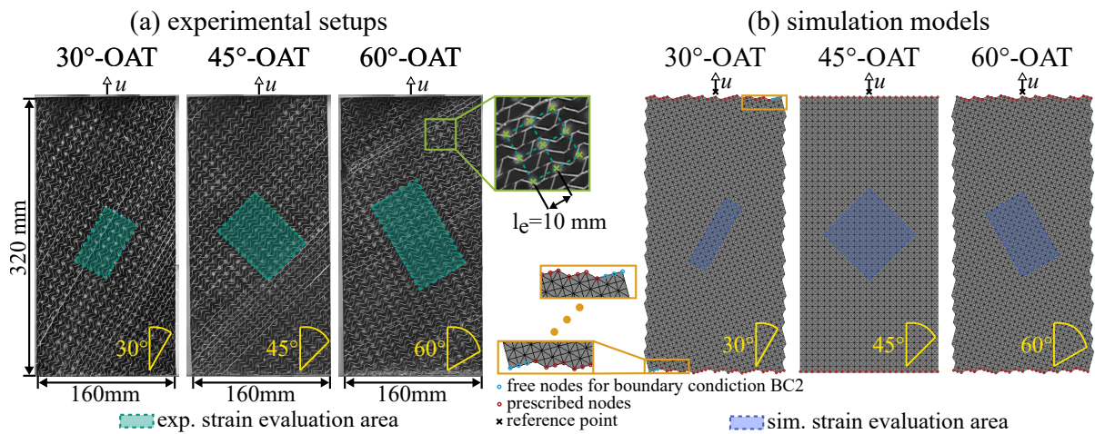
Fig. 2: (a) Experimental setups of the OATs with a square pattern of white points for optical measurements and highlighted areas (green) for an averaging of the strain components (based on [1]); (b) Simulation models with their respective boundary conditions to simulate slip in the clamping area during the 30°-OAT (boundary condition BC 2) and highlighted areas (blue) for an averaging of the strain components (based on [15])
