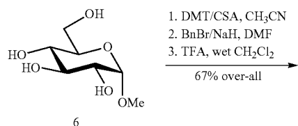
Scheme 1. Synthesis of monosaccharide-amino acid conjugate 10.
