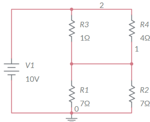
Figure 6. Schematic Diagram of an example circuit
