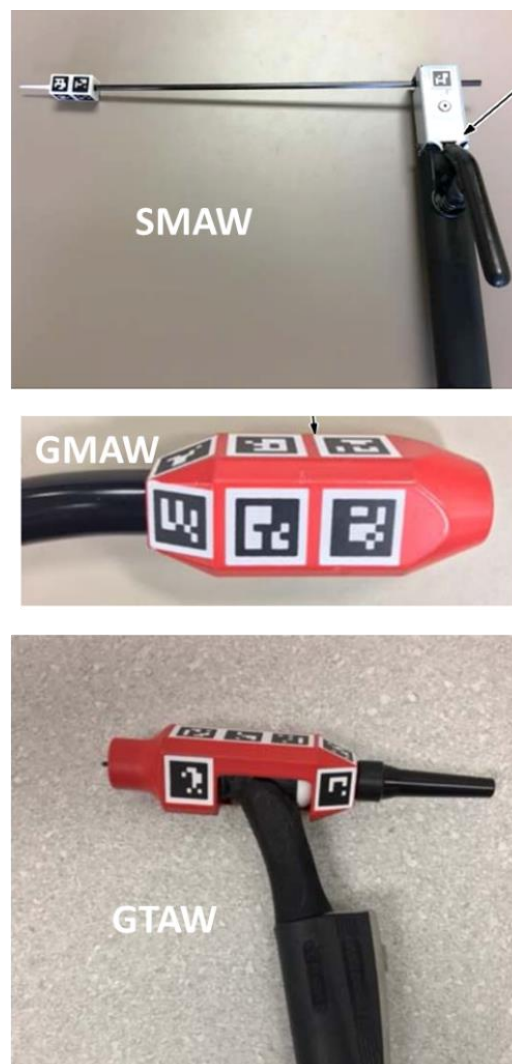
Figure 4: Augmented reality welding torches and electrodes for SMA, GTA ad GMA welding processes
