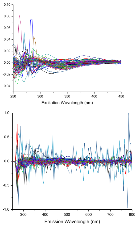
Figure S3: Residual plots for PARAFAC fit
