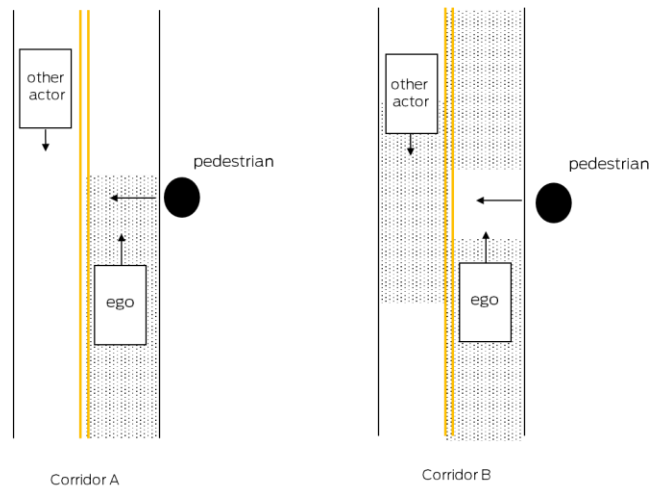
Figure 5 – Scenario 2 - example visualization of potential driving corridors in the case where a pedestrian enters the roadway and other actors are present. In this scenario, corridor B violates the duty of care owed to the other actor.
