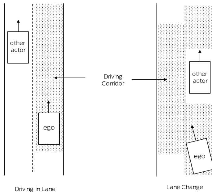
Figure 3 – Example visualization of the driving corridor used by the motion planner to determine violations of the various envelopes as it maneuvers.
