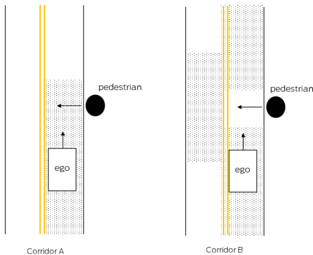
Figure 4 - Scenario 1– example visualization of potential driving corridors in the case where a pedestrian enters the roadway, and no other actors are present. In this scenario, corridor B allows for executable trajectories that avoid the imminent hazard without introducing duty of care violations to other road actors.
