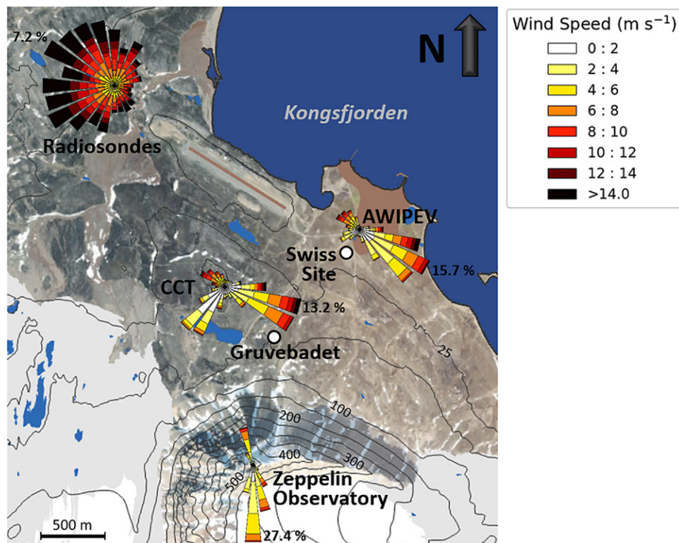
Fig. 4. Wind measurements during NASCENT throughout the Ny-Ålesund area at the different locations and retrieved from radiosondes. Data are shown for the AWIPEV weather mast (10 m), the Zeppelin Observatory, the CCT (10 m), and from daily radiosondes between 3,000 and 3,500 m MSL. The bar length gives the respective frequency of occurrence with the maximum frequency value specified at the end of the longest bar. The topographic map of the Ny-Ålesund region is from Norwegian Polar Institute (2014).
