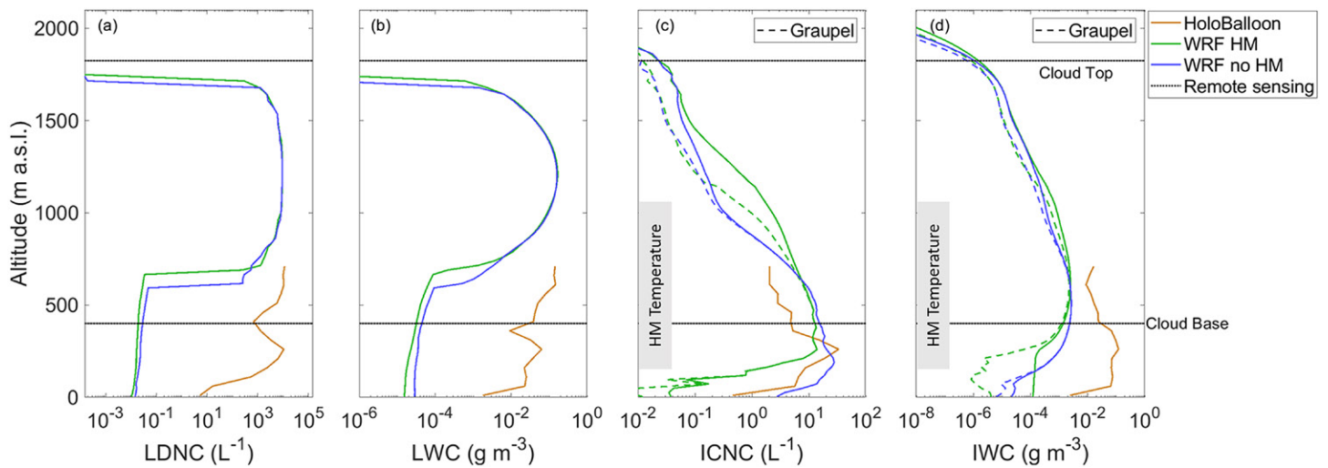
Fig. 12. The averaged vertical profiles during flight 3 on 12 Nov 2019 observed by HOLONO3B and simulated by WRF. (a) LDNC, (b) LWC, (c) ICNC, and (d) IWC. The contribution of graupel to the ICNC and IWC are shown with the colored dashed profile line in (c) and (d). The data from HOLONO3B are averaged over 50-m altitude bins and the WRF data over every model layer. The average cloud base and cloud top measured by the remote sensing instrumentation (ceilometer and cloud radar, respectively) are represented by the black dotted horizontal lines and the HM temperature range (from -8^{\circ} to -3^{\circ}\text{C} ) is highlighted in (c) and (d).
