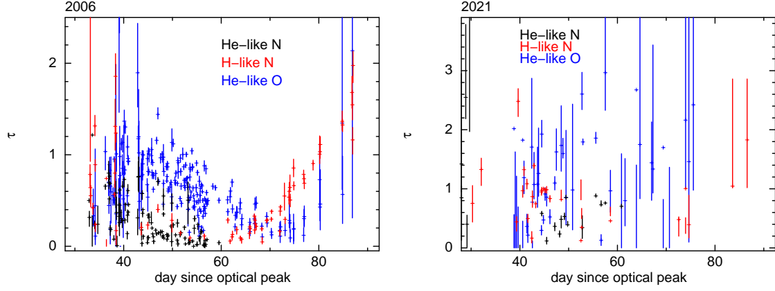
Figure 10. Plots of the fitted edge optical depths for which the 1\sigma lower limit is inconsistent with zero. For the 2006 dataset (left), the He-like O edge (0.739 keV; blue) was the most significant at early times, decreasing in strength with time. The shallower optical depth of the He-like N (0.552 keV; black) edge followed a similar decreasing trend. H-like N (0.635 keV; red) improved the fits mainly after day 60. The optical depths of the edges fitted to the 2021 spectra (right) do not show any obvious trends. The small number of edges for which the optical depth pegged at the deepest allowed value of \tau = 5 have been omitted from the plots. Note that the vertical scales are different for the two plots.
