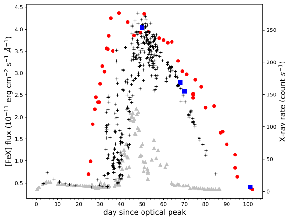
Figure 14. The evolution of the [Fe X] flux in 2021 and 2006 (red circles and blue squares; left-hand axis), compared with the corresponding 0.3–10 keV X-ray light-curves (grey triangles and black pluses; right-hand scale).
