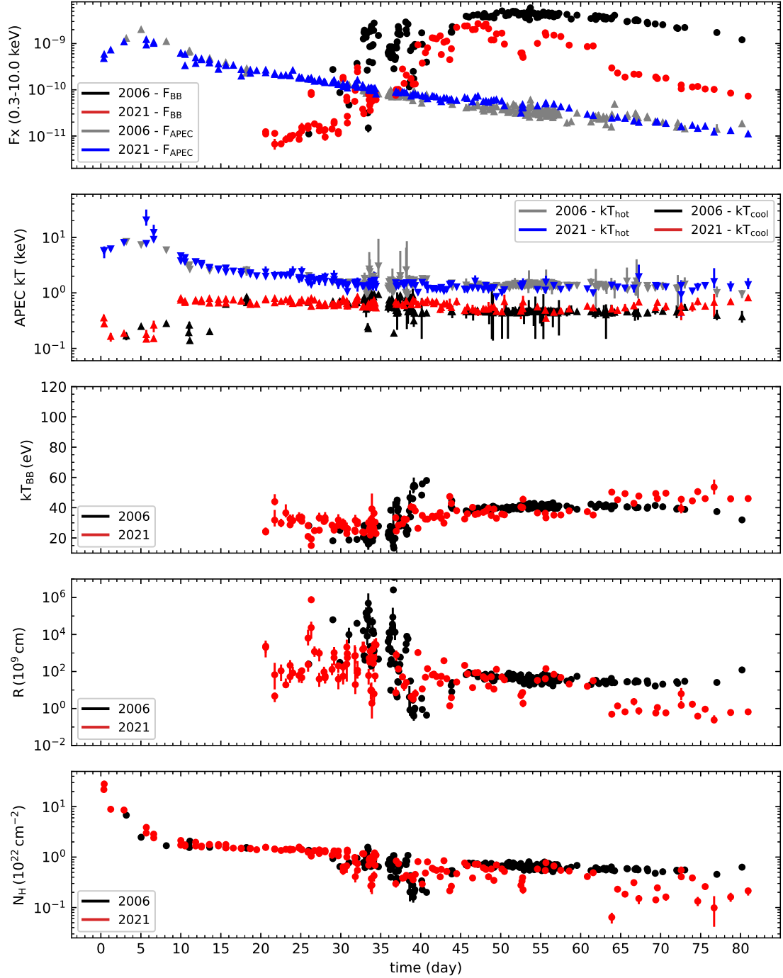
Figure 11. Results from fitting the spectra from 2006 and 2021 with a simple BB to model the soft emission, together with two optically-thin APEC components. The top panel shows the observed 0.3–10 keV fluxes from the BB and APEC components (in units of \text{erg cm}^{-2} \text{s}^{-1} ). The second panel shows the evolution of the APEC component temperatures, while the third panel shows the same for the BB. The fourth panel shows the emission radius for the BB component, and the bottom panel shows how the absorbing column N_{\text{H,wind}} (in excess of the Galactic ISM value) evolves with time. 2006 data are plotted in monochrome, while 2021 are in blue (hotter APEC parameters) and red (cooler APEC and all other parameters). Note that the ordinate scales are the same in each panel as in Fig. 12, for ease of comparison. See text for more details of the models.
