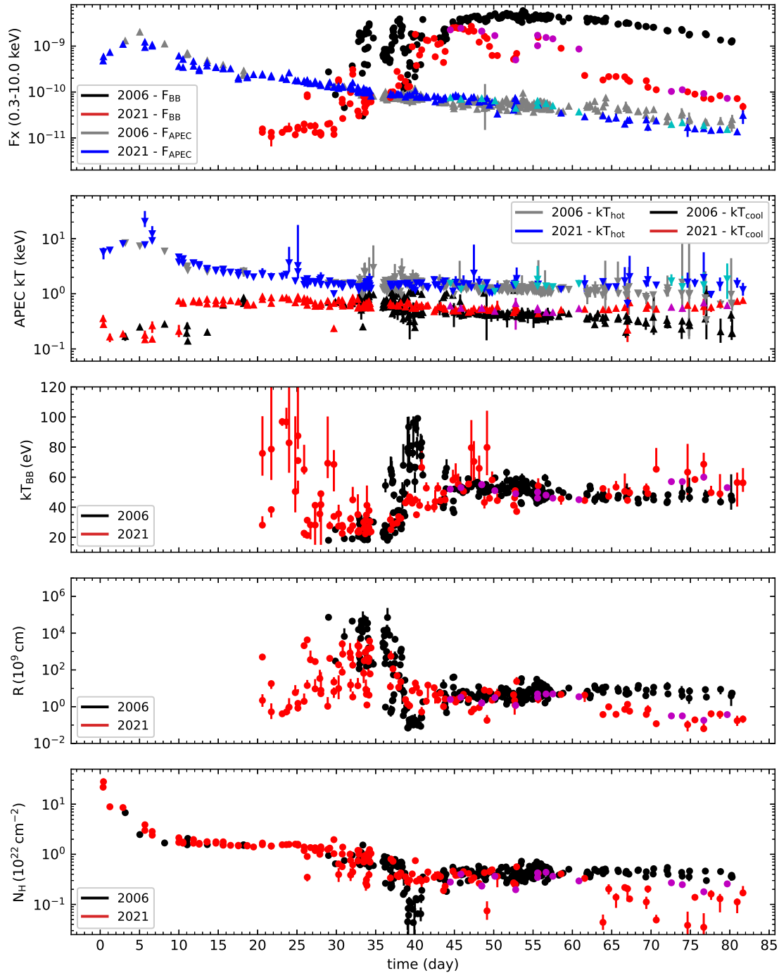
Figure 12. As for Fig. 11, but including four absorption edges as well. 2006 data are plotted in monochrome, while 2021 are in blue/cyan (hotter APEC parameters) and red/magenta (cooler APEC and all other parameters: red where BB kT was free to vary, magenta stars where that temperature was constrained). The APEC temperatures plotted in magenta and cyan correspond to the magenta BB bins, likewise for the radius and N_{\text{H}} . Note that the ordinate scales are the same in each panel as in Fig. 11, for ease of comparison. See text for more details of the models.
