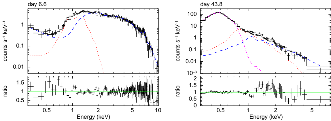
Figure 9. Example spectra demonstrating how well the models fit the 2021 data, before and during the SSS phase. Left panel: Spectrum from day 6.6 after the eruption, at the time the 1–10 keV emission peaked, fitted with two optically-thin components (red and blue). Right panel: Spectrum from day 43.8 after the eruption, around the time the 0.3–1 keV emission peaked, fitted with a blackbody plus edges (magenta), together with two optically-thin components (red and blue).
