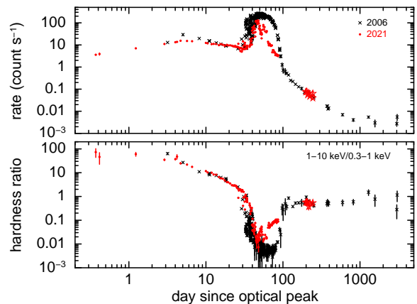
Figure 16. 0.3–10 keV light-curves from 2006 and 2021, including the post-SSS data. The red stars highlight the post-Sun-constraint observations in 2022 Feb.-Apr.
