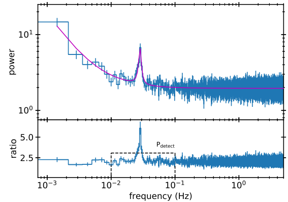
Figure 5. The upper panel shows the average of 59 periodograms (each spanning 700 s) from the 2021 WT data over days 36.87 – 61.56 (the main SSS interval), fitted with the model described in the text (magenta line). The bottom panel shows the ratio obtained between the average and model when the Lorentz (QPO) term is removed. The dashed line shows the 99 per cent detection level over the frequency range 0.01 – 0.10 Hz (i.e., periods of 10 – 100 s).
