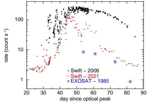
Figure 15. Comparison of the EXOSAT LE/LX3 observations following the 1985 eruption of RS Oph with the Swift light-curves from 2006 and 2021. The EXOSAT measurements have been converted to Swift -equivalent 0.3–1 keV count rates using WebPIMMS.
