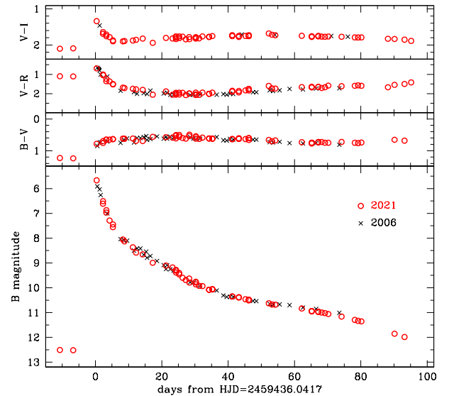
Figure 2. B -band photometry and colour diagrams from the ANS Collaboration, from both 2021 and 2006. The two outbursts are almost identical at optical wavelengths.
