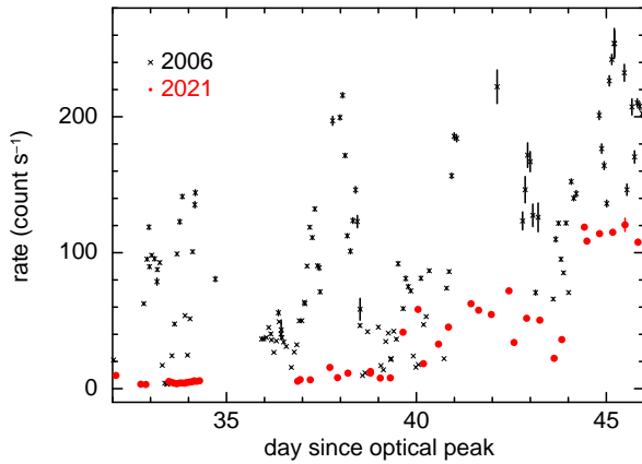
Figure 4. A comparison of the 2006 and 2021 0.3–1 keV light-curves during the early supersoft phase. The 2006 dataset reaches a higher count rate, and shows larger amplitude changes, though both datasets are variable. The peaks and troughs of the variability occur at different times in 2006 and 2021.
