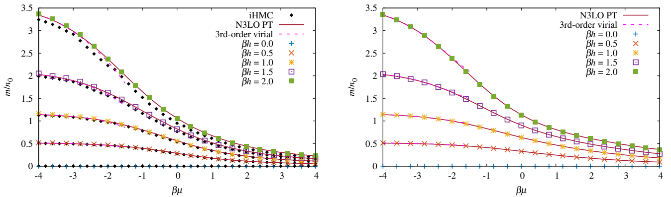
FIG. 2. Spin polarization m = n_{\uparrow} - n_{\downarrow} normalized by the noninteracting, unpolarized density n_0 for attractive (left) and repulsive (right) interactions of strength \lambda = \pm 1 . The CL results are shown with colored symbols, iHMC results (from Ref. [14]) appear with black diamonds, perturbative results at third order are shown with solid lines, and virial expansion results appear as dashed lines.
