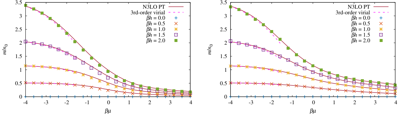
FIG. 5. Spin polarization m = n_{\uparrow} - n_{\downarrow} normalized by the noninteracting, unpolarized density n_0 for attractive (left) and repulsive (right) interactions of strength \lambda = \pm 2 . The CL results are shown with colored symbols, perturbative results at third order are shown with solid lines, and virial expansion results appear as dashed lines.
