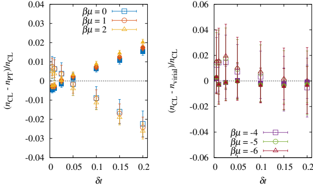
FIG. 3. (Left) Relative difference between the density n_{\uparrow} + n_{\downarrow} computed via CL ( n_{\text{CL}} ) and the third-order perturbative result n_{\text{PT}} for three positive values of \beta\mu , as a function of the CL time step \delta t . The dashed horizontal line shows where n_{\text{CL}} = n_{\text{PT}} . (Right) Relative difference between n_{\text{CL}} and the third-order virial expansion n_{\text{virial}} for three values of \beta\mu of small fugacity, as a function of \delta t . The dashed horizontal line shows where n_{\text{CL}} = n_{\text{virial}} . In both plots, the coupling was set to \lambda = \pm 1 , where solid and open symbols refer to repulsive and attractive couplings, respectively. Error bars represent the statistical error of the CL calculation, and indicate agreement with PT and the virial expansion as \delta t \rightarrow 0 .
