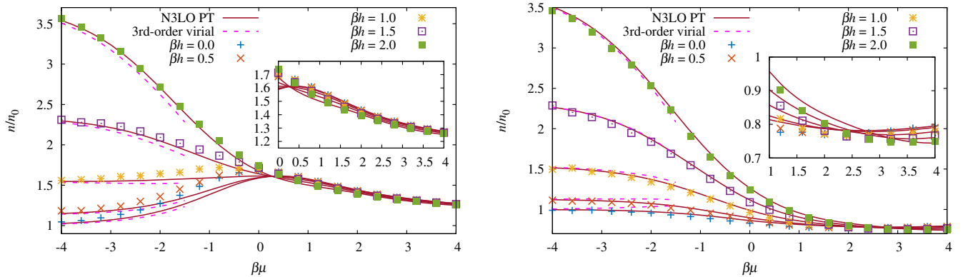
FIG. 4. Density equation of state n = n_{\uparrow} + n_{\downarrow} normalized by the noninteracting, unpolarized counterpart n_0 for attractive (left) and repulsive (right) interactions of strength \lambda = \pm 2 . Insets: Zoom in on the region \beta\mu > 0 (left) and \beta\mu > 1 (right). The CL results are shown with colored symbols, perturbative results at third order are shown with solid lines, and virial expansion results appear as dashed lines.
