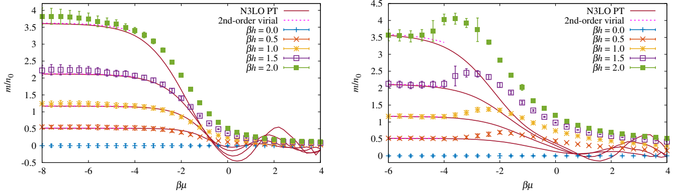
FIG. 7. Spin polarization m = n_{\uparrow} - n_{\downarrow} normalized by the noninteracting, unpolarized density n_0 for attractive (left) and repulsive (right) interactions of strength \lambda = \pm 4 . N3LO perturbation theory no longer offers a viable comparison for the polarization at this coupling strength, except near the virial region.
