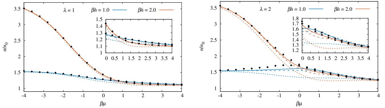
FIG. 8. Density n = n_{\uparrow} + n_{\downarrow} normalized by the noninteracting, unpolarized counterpart n_0 for attractive interaction of strength \lambda = 1 (left) and \lambda = 2 (right). The CL results are shown with black diamonds, perturbative results at first (NLO), second (N2LO), and third (N3LO) order are shown with dotted, dashed, and solid lines, respectively.
