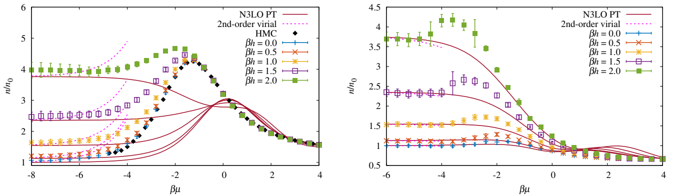
FIG. 6. Density equation of state n = n_{\uparrow} + n_{\downarrow} normalized by the noninteracting, unpolarized counterpart n_0 for attractive (left) and repulsive (right) interactions of strength \lambda = \pm 4 . The CL results are shown with colored symbols, perturbative results at third order are shown with solid lines, and HMC for the attractive, unpolarized case is shown in black diamonds [44].
