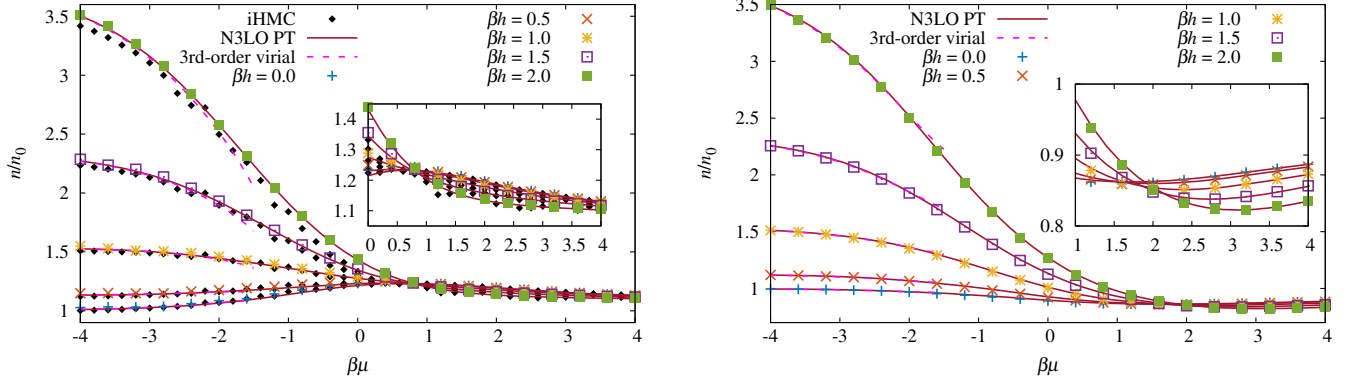
FIG. 1. Density equation of state n = n_{\uparrow} + n_{\downarrow} normalized by the noninteracting, unpolarized counterpart n_0 , for attractive (left) and repulsive (right) interactions of strength \lambda = \pm 1 . Insets: Zoom in on the region \beta\mu > 0 (left) and \beta\mu > 1 (right). In all cases, the CL results are shown with colored symbols, iHMC results (from Ref. [14]) appear with black diamonds, perturbative results at third order are shown with solid lines, and virial expansion results appear as dashed lines.
