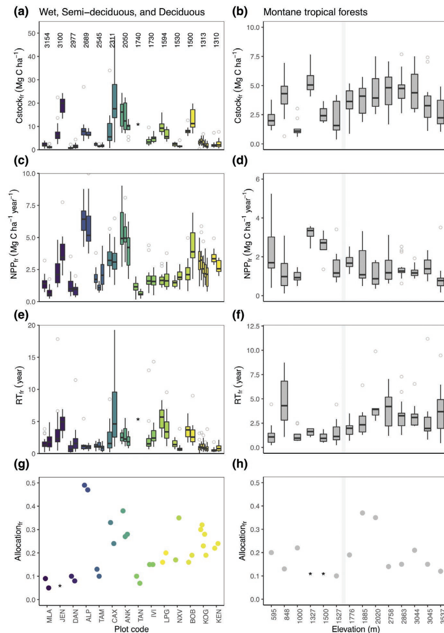
FIGURE 2 Variation in lowland (left) and montane (right) tropical forests of (a, b) total fine root carbon stock ( \text{Cstock}_{\text{fr}} ), (c, d) fine root net primary productivity ( \text{NPP}_{\text{fr}} ), (e, f) fine root residence time ( \text{RT}_{\text{fr}} ), and (g, h) the fractional carbon allocation of total ecosystem NPP to fine roots ( \text{Allocation}_{\text{fr}} ). Wet (3154–2050 \text{mm year}^{-1} ), semi-deciduous, and deciduous (1740–1310 \text{mm year}^{-1} ) lowland forests (left panels) are ordered from highest (left) to lowest (right) mean annual precipitation ( \text{mm year}^{-1} ), which is shown on the upper x-axis. The montane tropical forests (right panels) are ordered from lowest to highest elevations and grey shaded area indicates the cloud base at 1600 m a.s.l. (consistent with Malhi et al., 2017). Forest type designations of the plots followed Rifai et al., (2018). Note the different y-axis scales for lowland and montane forests. In some tropical forests, some aspects of fine root dynamics data were not recorded and missing data are denoted with an asterisk (*). For the list of the plots and their characteristics, see Table 1
