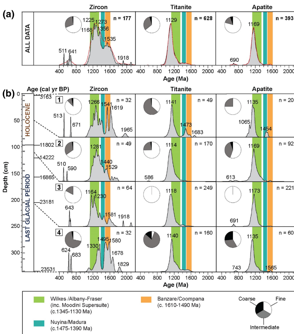
Figure 5. Detrital age signatures in KC14. (a) Age spectra for detrital zircon, titanite, and apatite for the entire KC14 core presented as probability-density plots (black curve, gray fill). Kernel density curve is shown in red. (b) Probability-density plots showing downcore age variability in detrital zircon, titanite, and apatite. Gray rectangles within the stylized core on left hand side show where sediment samples were taken from within each depth interval of KC14 for U-Pb analysis. Major age peaks and total number of analyses ( n ) are indicated. Age signatures of geological provinces in East Antarctica/southern Australia (as in Figure 2) are highlighted as colored bars for comparison. Although the Moodini Supersuite intrudes the Banzare/Coompana and Nuyina/Madura provinces, it is here grouped with the Wilkes Province/Albany-Fraser Orogen due to the overlap in age ranges. Pie charts show relative proportion of each mineral size fraction contributing to the age signature for each depth interval. Intervals 1–4 represent changes in biogenic silica concentration and are the same as those presented in Figure 3.
