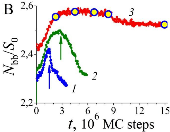
(B) Change in time of the number of broken bonds on the surface of nanowires for the same parameters. S_0 is the side surface area of the nanowire in dimensionless units in initial state. The arrows indicate the moments of the first ruptures in the nanowires. The circles on curve 3 mark the moments of time for which in Figure 8C the shapes of the thickest nanowire are shown.
