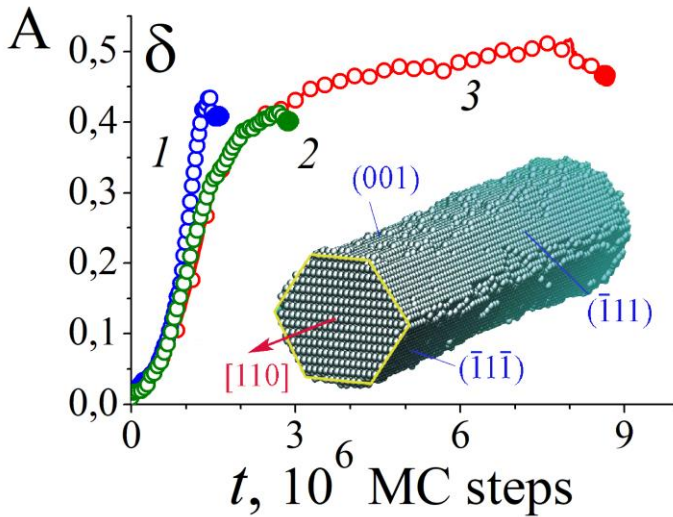
Figure 7: Dynamics of morphology characteristics of nanowires with [110] orientation under stimulation of atomic surface diffusion. \alpha = 1 , p = 0.825 . (A) Change in the level of modulation of the cross section of nanowires, ( \delta ), of different radii. For curves 1, 2, 3 – r_{nw} = 15.5 , L = 700 ; r_{nw} = 17.5 , L = 700 ; and r_{nw} = 20.5 , L = 500 respectively. Color circles mark the time moments of the first ruptures. The inset shows the typical shape of a nanowire with [110]-orientation established at the initial stage of its transformation.
