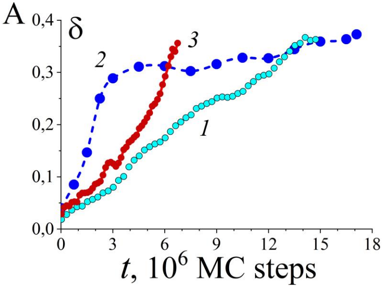
Figure 6: Dynamics of nanowires with [100] orientation in different regimes. (A) Dependencies of the level of modulation of the cross section of the nanowire, \delta(t) , on time: \delta = \langle \Delta N_{layer}^2 \rangle / \langle N_{layer} \rangle^2 , N_{layer} is a number of atoms in transverse atomic layers. Initial nanowire radius r_{nw} = 15.5 , length L = 700 . Curve 1 (cyan circles) - p = 0.7, \alpha = 1 (breakup without external irradiation). Blue circles - p = 0.825, \alpha = 1 (transformation under external irradiation without heating). Red curve (3) - p = 0.825, \alpha = 0.8 (breakup under external irradiation with heating). Dependences \delta(t) are given up to the first nanowire rupture.
