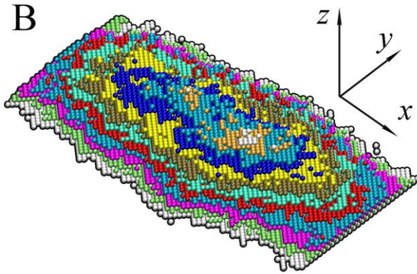
B – A typical hillock having formed on the side nanowire surface by the time moment t = 3 \times 10^6 MC time steps. The sizes of the lowest (001)-layer (marked in red) are around l_x \sim 53a , l_y \sim 23a .
