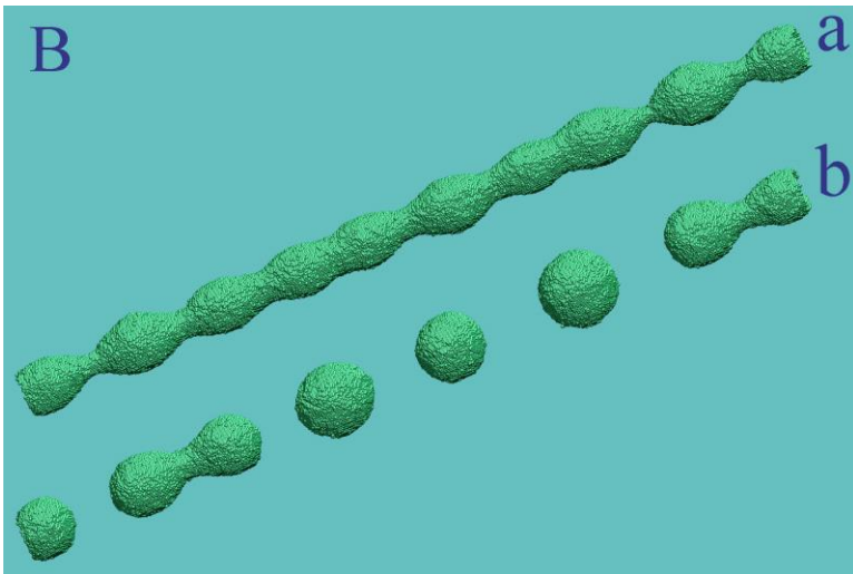
(B) - r_{nw} = 17.5 , L = 700 ; (a), (b) - t = 2.70 and 5.88(\times 10^6) MC steps.
