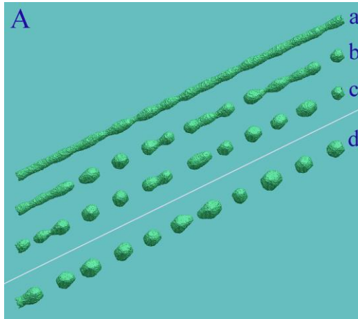
Figure 10: Breakup of nanowires with [111] orientation without external irradiation (subpart (A)) and under conditions of stimulated surface diffusion of atoms (subpart (B)). (A) \alpha = 0.9 , p = 0.725 , L = 1050 . Configurations (a), (b), (c) - r_{nw} = 12.5 ; t = 3.0, 4.2, 5.4(\times 10^6) MC steps. Configuration (d) - r_{nw} = 14.5 ; t = 9.45(\times 10^6) MC steps.
