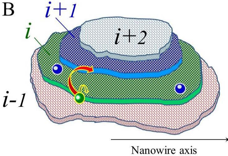
Figure 3: Scheme of a fragment of a modulated nanowire (A) and a hillock (B) for estimating the calculation of the balance of surface fluxes of atoms from layer i to layer (i + 1) and back. In subsection B, long jumps marked in red are prohibited.
