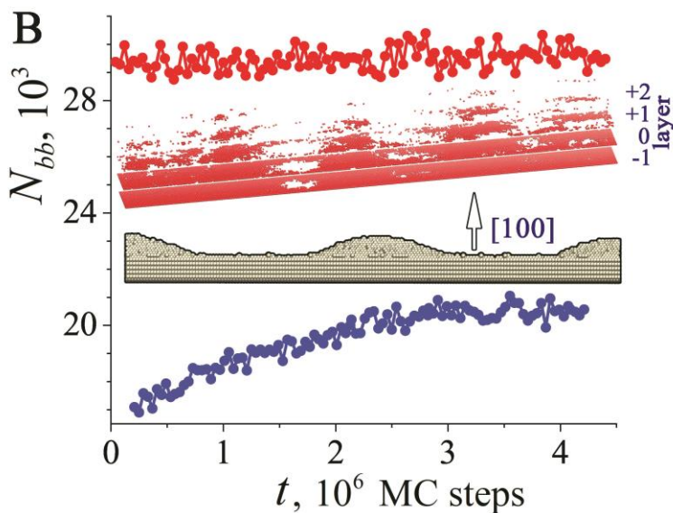
(B) Results for (100)-orientation of the upper face of the plate. L = 550, w = 70, h = 10 . The blue and red circles show time dependencies, N_{bb}(t) , for cold and hot regimes respectively. In cold regime, six hillocks with a height of 8-10 atomic layers are formed on the upper plane. Bottom inset presents a fragment of the plate. In the hot regime, only two or three near-surface atomic layers are partially filled (upper inset). The observed low structuredness of the surface is characterized by longer wavelength perturbations.
