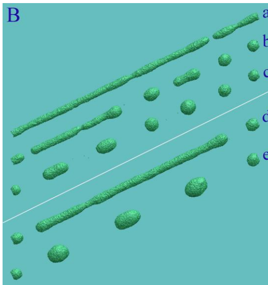
(B) - \alpha = 0.9 , p = 0.8 , L = 1050 . Configurations (a), (b), (c) - r_{nw} = 12.5 ; t = 3.0, 4.8, 7.2(\times 10^6) MC steps. Configurations (d), (e) - r_{nw} = 14.5 ; t = 12.0, 26.1(\times 10^6) MC steps.
