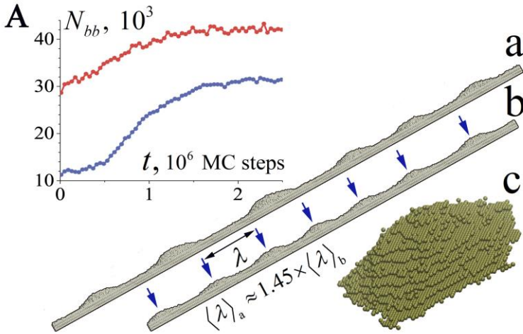
Figure 5: Effect of possible surface heating on the manifestation of stimulated roughening transition on faces of different orientations.
