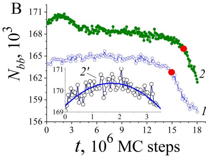
(B) Variations in time of the number of broken bonds, N_{bb}(t) , for surface atoms of the nanowire. The parameters for curves 1 and 2 are the same as for curves 1 and 2 presented in Subpart A. The lower inset, curve 2', represents the initial stage of dependency 2.
