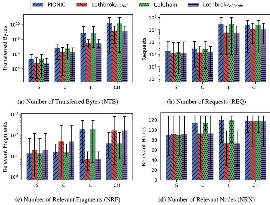
Fig. 20. Number of Transferred Bytes (NTB) (a), Number of Requests (REQ) (b), Number of Relevant Fragments (NRF) (c), and Number of Relevant Nodes (NRN) (d) for each LARDFBench query load.
