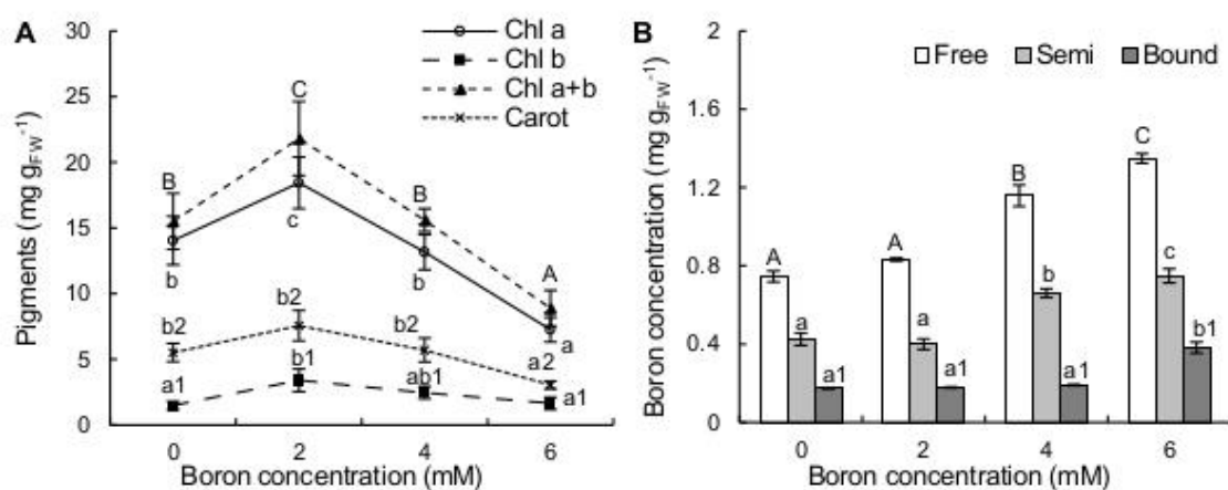
Fig. 2. Photosynthetic pigments (chl a ; chl b ; chl a + b ; carot; A) and boron concentration (free, semi-bound; and bound B) in tomato seedlings grown under 0, 2, 4, and 6 mM boron for 20 days. The data are means \pm SD ( n = 4 ). Different letters, capital for chl a , free B and small for chl b , semi-bound B, small 1 for chl a + b , bound B, small 2 for carot, indicate statistically significant differences ( P \leq 0.05 ).
