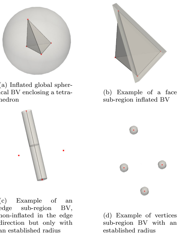
Fig. 12 Examples of BV employed for global contact-search
