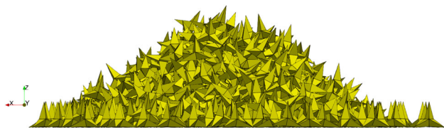
Fig. 28 Lateral view of the final configuration obtained after collapsing the box of tetrapods
