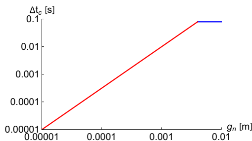
Fig. 11 Critical time-step \Delta t_c considering interface law of Fig. 10b, considering forces in N, displacements in m and an equivalent mass of 156.594 kg
