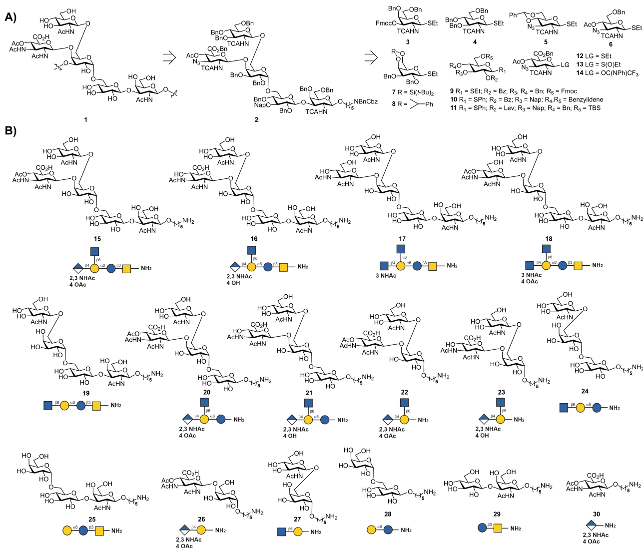
Figure 2. A) Repeating unit of A. baumannii 17978 CPS and related oligosaccharides synthesized from building blocks 3–14 ; B) Structure of A. baumannii 17978 related glycans 15–30 . TCA = trichloroacetyl; N 3 = azide; Ac = acetyl; Bn = benzyl, Bz = benzoyl, TBS = tert -butyldimethylsilyl, Nap = 2-naphthylmethyl; Lev = levulinyl; Fmoc = fluorenylmethyloxycarbonyl; Cbz = carboxybenzyl; Ph = phenyl.
