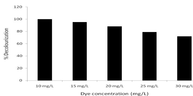
Figure 4: Effect of dye concentration on decolourization by binary mixed culture of P. fluorescense and A. niger
