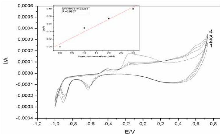
Fig 3. Cyclic voltammograms of copper oxides-copper electrode in 0.1 M NaOH (supporting electrolyte) and in the presence of various concentrations of urate: 1-0; 2-1mM; 3-2 mM; 4-3 mM; starting potential:-0.221V vs SCE; potential range: -0.221 → +0.75 → -1V vs SCE; scan rate: 0.05 V/s; 5 th scan
