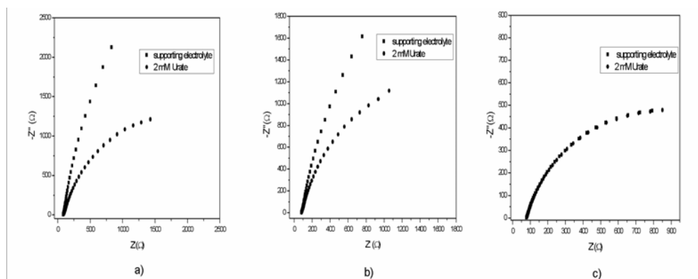
Fig 5. The experimental Nyquist diagrams at different potential value of a copper electrode in 0.1 M NaOH in absence/presence of urate: a) E=0.4 V vs SCE; b) E=0.5 V vs SCE; c) E=0.6 V vs SCE
