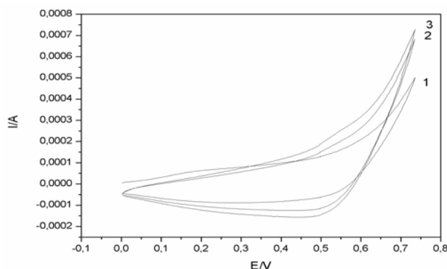
Fig 2. Cyclic voltammograms of copper oxides-copper electrode in 0.1 M NaOH and 2 mM urate after preanodization of copper electrode at + 2.5V vs SCE for the time of 2 minutes; starting potential: 0.00V vs SCE; potential range: 0.00 → +0.75 → 0.00 V vs SCE; scan rate: 0.05 V/s; 1- 1 st scan, 2-3 rd scan, 3-5 th scan
