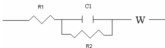
Fig 6. The equivalent circuits to fit the EIS for copper oxide electrodes in the absence/presence of urate in aqueous 0.1 M NaOH solution
