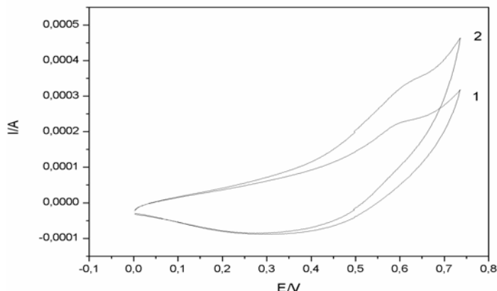
Fig 4. Cyclic voltammograms of copper oxides electrode in 0.1 M NaOH as supporting electrolyte and in the presence of : 2 mM urate (curve 1); 2mM urate and 2 mM tartrate (curve 2); starting potential: 0.00V vs SCE; potential range: 0.00 → +0.75 → 0V vs SCE; scan rate: 0.05 V/s; 5 th scan
