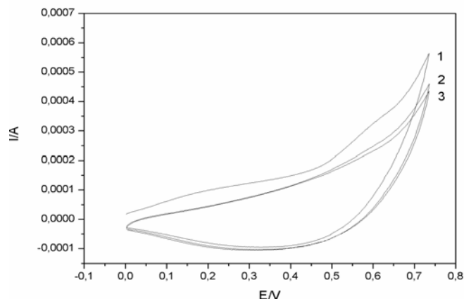
Fig 1. Cyclic voltammograms of copper oxides-copper electrode in 0.1 M NaOH and 2 mM urate after copper electrode cycling (5 scans) under the same conditions but in the extended potential range ( -0.221 \rightarrow +0.75 \rightarrow -1.00 V vs SCE); starting potential: 0.00V vs SCE; potential range: 0.00 \rightarrow +0.75 \rightarrow 0.00 V vs SCE; scan rate: 0.05 V/s; 1- 1 st scan, 2-3 rd scan, 3-5 th scan
