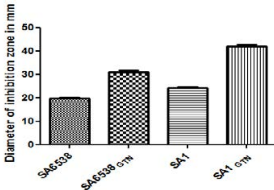
Figure 3. Reduction of tolerance to oxidative stress by ¼ MIC of GTN. *, significant P < 0.05.
