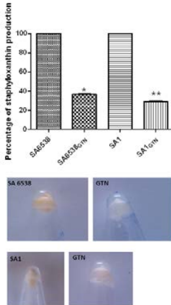
Figure 2. Inhibition of Staphyloxanthin production by \frac{1}{4} MIC of GTN. *, significant P < 0.05 .
