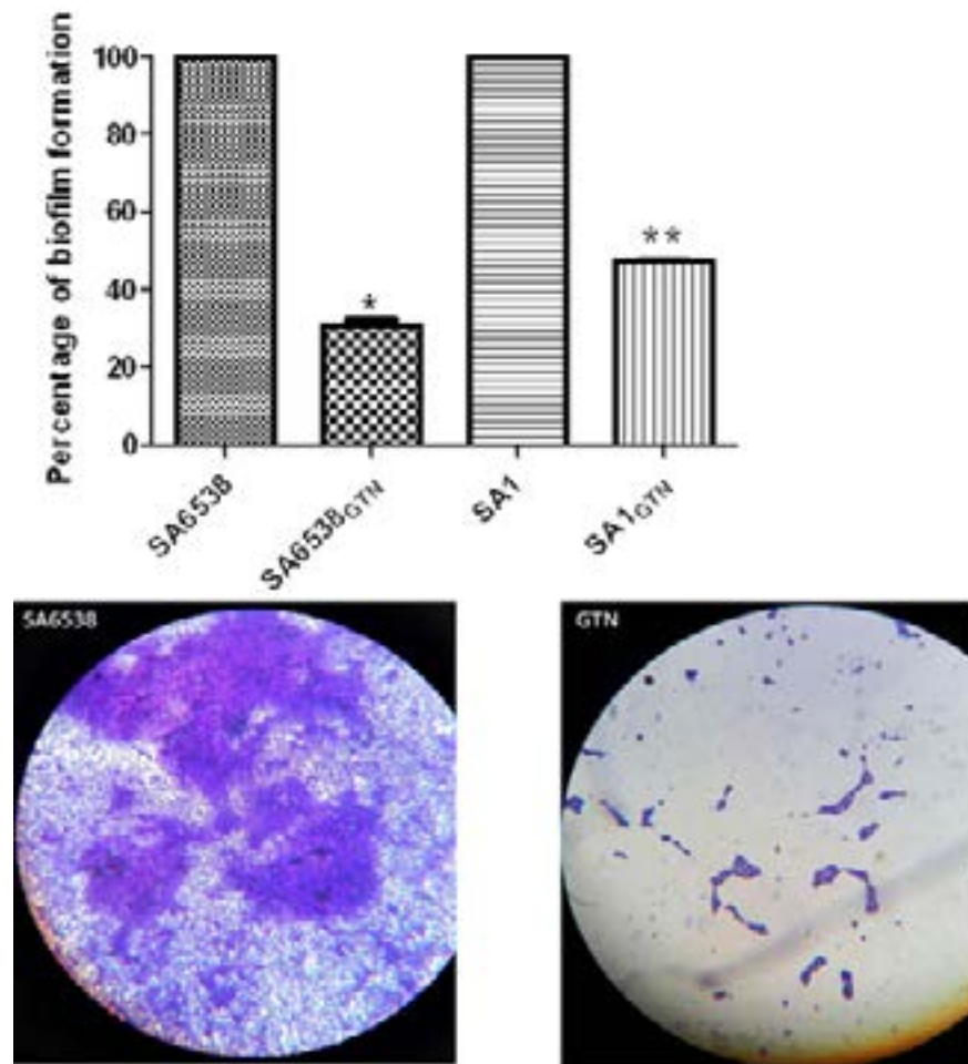
Figure 1. Inhibition of biofilm formation of S. aureus by ¼ MIC of GTN. *, significant P < 0.05. Microscopic images of biofilm formed by S. aureus ATCC 6538 under the light microscope (X400) in the treated culture (right) and untreated (left).
